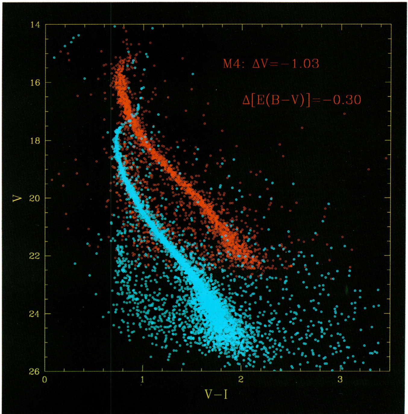
FIG. 2.—M4 data ( red ) have been overlayed on the M55 data ( blue ) after applying the indicated vertical and horizontal shifts, which ensure that the Galactic bulge stars in the two fields have the same reddening and apparent distance modulus. See the text for additional discussion.
