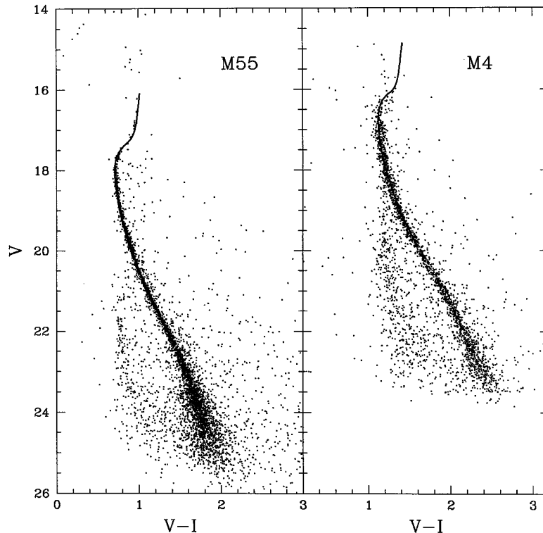
FIG. 1.—CMDs for M55 and M4 are shown. The solid lines are 16 Gyr isochrone fits with \text{Fe}/\text{H} = -1.77 and \text{Fe}/\text{H} = -1.27 for M55 and M4, respectively. See the text for discussion of the background sequences visible in each field.
