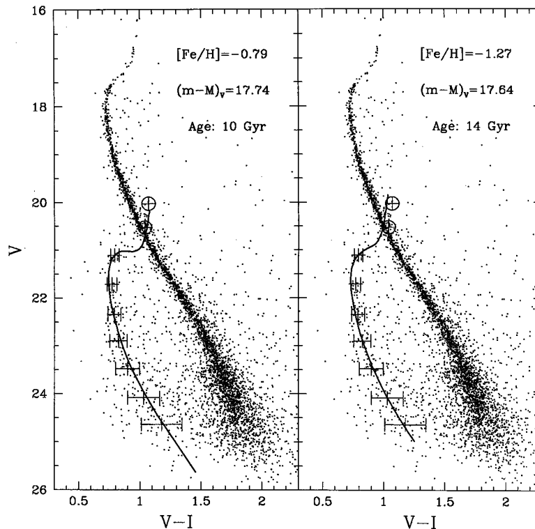
FIG. 3.—M55 data (points) are plotted together with the ridge line of the SDG MS (points with error bars) and two subgiant points from SL (circled crosses). The VB85 isochrones with the indicated metallicity, apparent distance modulus, and age have been overlayed on the SDG sequence. In each case, the applied reddening has been fixed at E(B - V) = 0.14 , the value used for the isochrone fit to M55 itself shown in Fig. 1.
