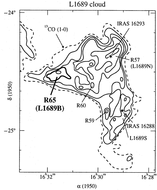
Fig. 1. Large-scale spatial distribution of the (low-density) molecular gas in the L 1689 cloud (adapted from Fig. 3c of Loren 1989a). The contours represent the ^{13}\text{CO}(1-0) line intensity measured at V_{\text{LSR}} = 3.83 km s ^{-1} by the MWO 4.9 m telescope ( 2.4' beam) and go from T_R^* = 2 K (dashed line) to T_R^* = 12 K by steps of 2 K. The L 1689B core studied in this paper is embedded within the clump denoted R65 by Loren.
