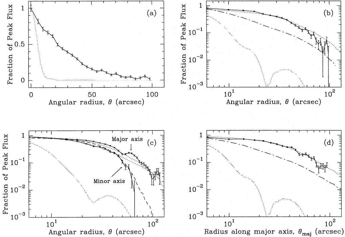
Fig. 3a–d. Normalized radial flux-density profiles of the L 1689B core (solid lines) obtained by averaging the observed 1.3 mm emission under circular (a,b) or elliptical (c,d) symmetry assumptions. In all panels, the beam profile is shown as a light dotted line for comparison. a Azimuthally-averaged profile in linear-linear format. b Azimuthally-averaged profile in log-log format compared to the simulated profiles of two model sources. The dash-dotted line corresponds to a model of the form I(\theta) \propto \theta^{-1} down to \theta = 1'' . The dotted line represents a model such that I(\theta) \propto \theta^{-0.3} for \theta \leq 25'' and I(\theta) \propto \theta^{-1} for \theta \geq 25'' . c Log-log intensity profiles along the major (upper solid curve) and minor (lower solid curve) axes of the core, obtained by azimuthally averaging the signal observed in the smoothed map of Fig. 2 over 40^\circ sectors. These observed profiles are compared with the similarly averaged major and minor profiles of an elliptical model of aspect ratio 0.7 such that I(\theta_{maj}) \propto \theta_{maj}^{-0.3} for \theta_{maj} \leq 25'' and I(\theta_{maj}) \propto \theta_{maj}^{-1} for \theta_{maj} \geq 25'' (dotted lines). The dashed line shows the simulated profile of a 57'' (FWHM) Gaussian model which fits most of the minor axis profile of L 1689B. d Elliptically-averaged intensity profile in log-log format, compared with simulated profiles (dotted and dashed-dotted lines) corresponding to elliptical models with the same angular dependence along their major axis as the models shown in b . A position angle of 90^\circ and an aspect ratio of 0.7 were assumed for the elliptical averaging.
