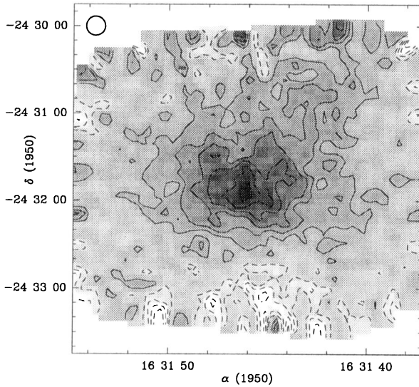
Fig. 2. “On-the-fly” 1.3mm continuum map of the prestellar core L 1689B obtained with the MPIR 7-channel/19-channel arrays in Feb./March 1995. This map results from the combination of 11 multi-channel coverages and was smoothed to an effective angular resolution of 13''. Contour levels go from −40 to −10 mJy/beam (dotted lines) and from 10 to 60 mJy/beam (solid lines) with steps of 10 mJy/beam. The rms noise level is ~ 3 mJy/13'' beam. The effective FWHM beam size is shown in the upper left corner.
