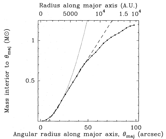
Fig. 4. Mass contained within ellipses of aspect ratio 0.7 and major radius \theta_{\text{maj}} as a function of \theta_{\text{maj}} . The mass was estimated from the flux mapped at 1.3 mm with 11'' resolution assuming T = 18 K and \kappa_{1.3} = 0.005 \text{ cm}^2 \text{ g}^{-1} (see text). The dotted and dashed lines show the relations M \propto \theta_{\text{maj}}^2 and M \propto \theta_{\text{maj}} which best approach the observations for \theta_{\text{maj}} < 25'' and \theta_{\text{maj}} > 25'' , respectively. The dashed, straight line represents our best estimate of the outer mass profile after correction for the loss of flux occurring at large angular radii.
