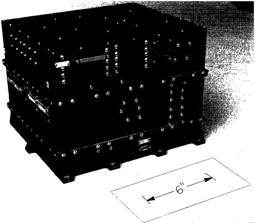
Fig. 5. A photograph of the main PWI electronics package.
