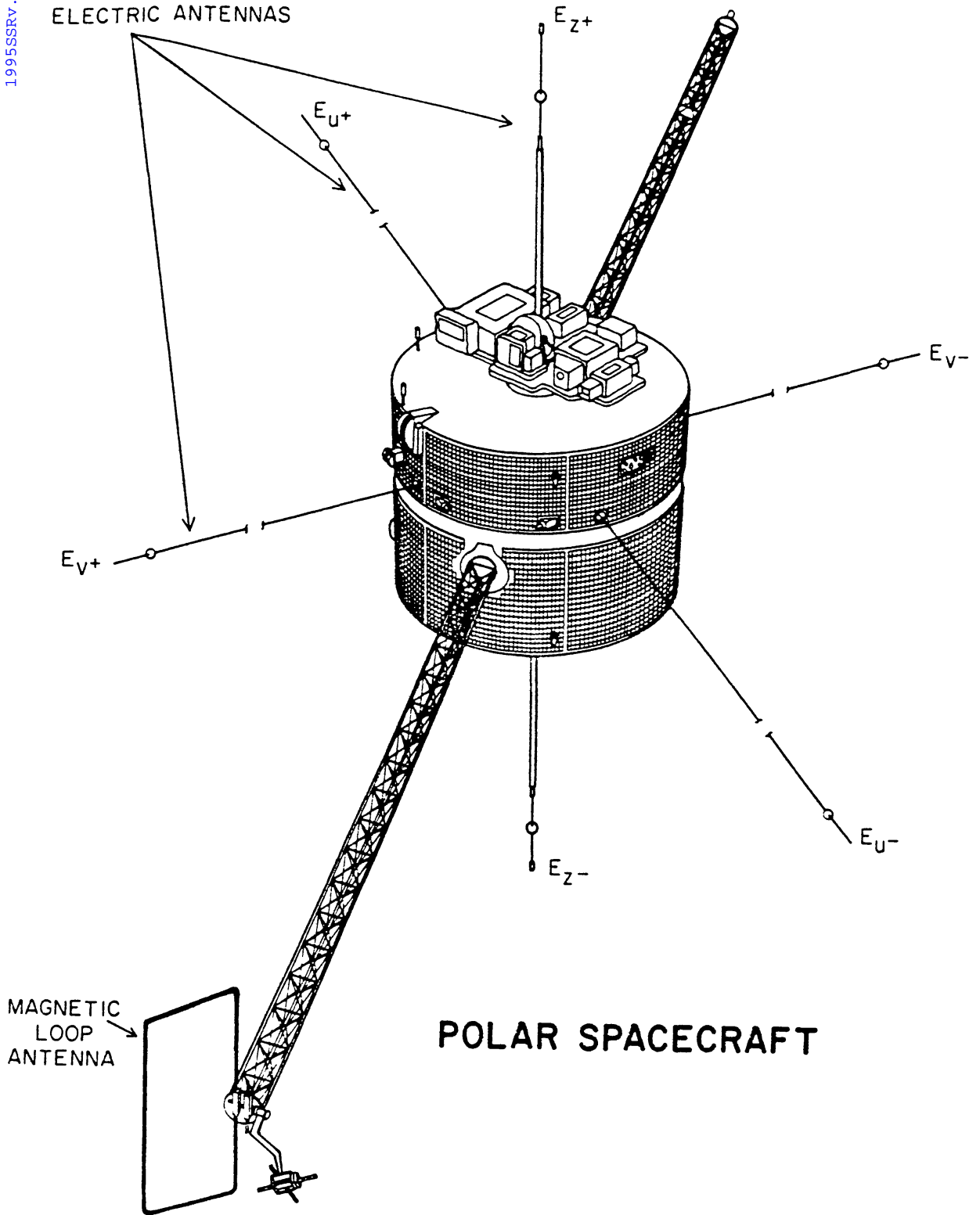
Fig. 1. A schematic drawing of the Polar spacecraft, illustrating the orientation of the three orthogonal electric antennas, the magnetic loop antenna, and the triaxial search coil antennas.
