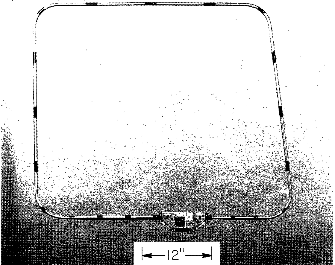
Fig. 3. A photograph of the magnetic loop antenna.
