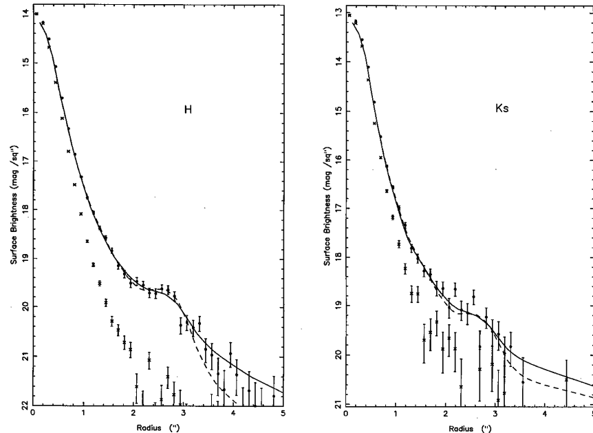
FIG. 2.—Azimuthally averaged radial profiles for the H -band mosaic (left) and the K_s mosaic (right). The upper points (circles) are for PG 1545+210; the lower points (crosses) are for the PSF. The profile of the latter has been normalized to that of the quasar. The solid line represents the best fit to a de Vaucouleurs-model profile while the dashed line represents the best fit to an exponential disk profile.
