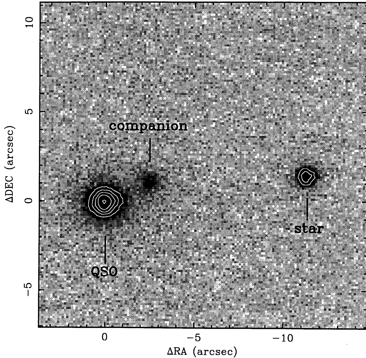
FIG. 1.—Mosaic of H -band images of PG 1545+210 taken with the 200 inch telescope. North is up and east is to the left. Contours are logarithmic, each a factor of 2 above the previous one. The highest contour level is \sim 95\% of the peak emission of the quasar. The companion galaxy west and slightly north of the quasar is evident. The star \sim 11''.4 to the west illustrates the quality of the seeing.
