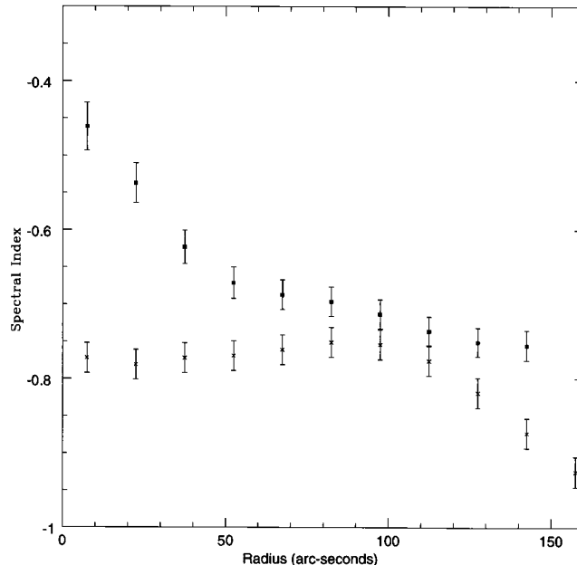
FIG. 8.—Plot of spectral index as a function of radius between 74 and 333 MHz (filled squares) and 333 and 1381 MHz (crosses). The plotted points are average values within concentric annuli of width and separation 15'' . Error bars are 1\sigma uncertainties based on the rms errors in the flux density maps added in quadrature with the quoted 2% uncertainty in the Baars et al. (1976) spectrum of Cas A, then propagated through to the spectral index calculation. R = 0'' was defined at the geometric center of Cas A's bright radio ring as determined from higher resolution radio studies (Rudnick 1995).
