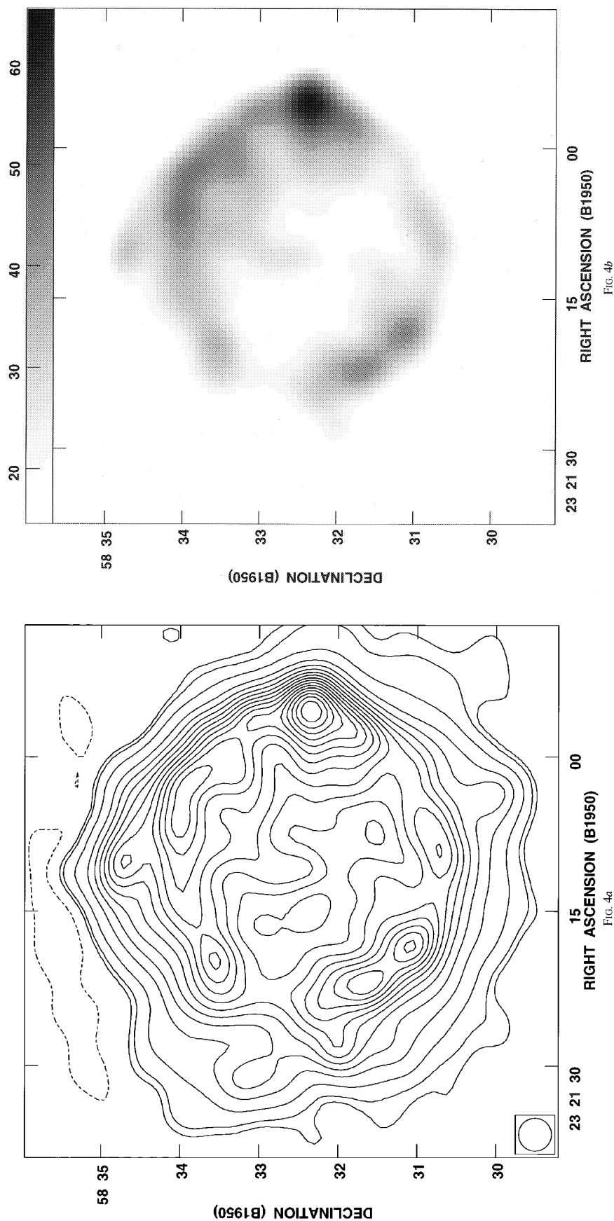
FIG. 4.—Contour ( a ) and gray-scale ( b ) flux density plots of the SNR Cas A at 1381 MHz, courtesy of L. Rudnick. The peak brightness temperature is 63.2 \text{ Jy beam}^{-1} , and the rms noise \sigma is \sim 135 \text{ mJy beam}^{-1} . The angular resolution is 25'' and is shown at the lower left. Contours in ( a ) are at (-3, -3, 6, 20, 50, 80, 110, 140, 170, 200, 230, 260, 290, 320, 350, 380, 410, 440) \sigma . For ( b ) the gray-scale flux density range is from 15 to 65 \text{ Jy beam}^{-1} , as indicated by the scale at the top of the image.
