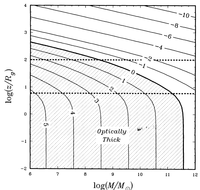
FIG. 3.—Contour plot of the log of the \gamma - \gamma optical depth \tau_{\gamma\gamma} (eq. [4.3]) for \gamma -rays with energy E = 1 GeV created at height z above the center of a two-temperature disk ( \omega = 3 ) with outer radius R_0 = 30R_g and inner radius R_{\text{ms}} = 6R_g . The upper and lower dashed horizontal lines denote z = R_0 and z = R_{\text{ms}} , respectively, and the \gamma -rays propagate outward along the z -axis. The curves were computed using the X-ray data for 3C 279 taken during the 1991 June EGRET flare by Makino et al. (1993).
