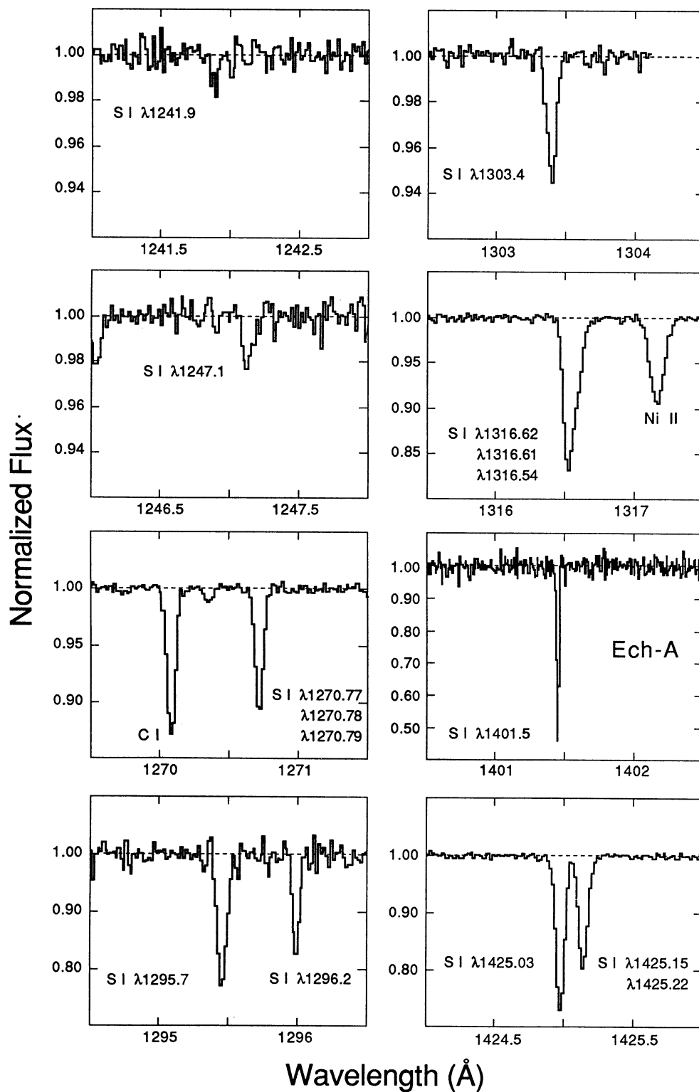
FIG. 2.—Newly analyzed S I lines. The line at 1401.5 \text{ \AA} comes from echelle data; the others are from spectra acquired with G160M. Features ascribed to multiple lines are blends. The lines of C I and Ni II in these spectral ranges are also noted.
