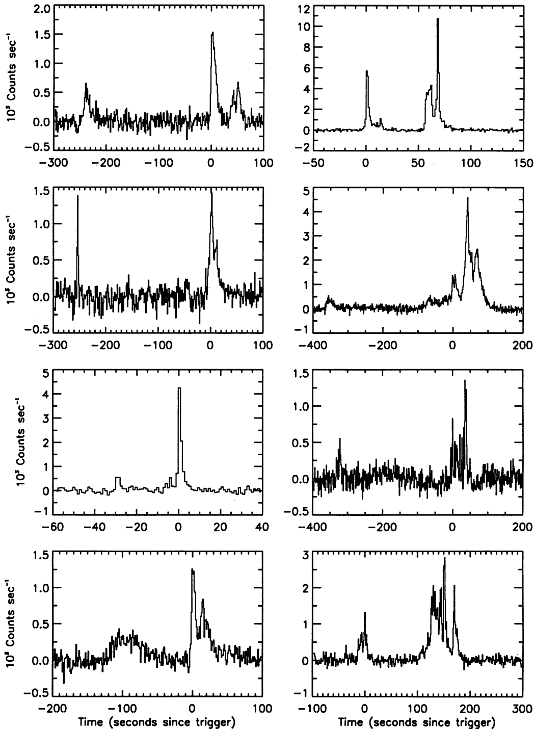
FIG. 3.—Time profiles, observed at energies > 20 keV, of the 24 bursts that have met the requirements for precursor activity. The time resolution of the data is 1.024 s.
