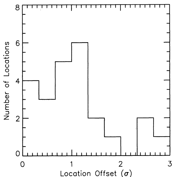
FIG. 2.—Distribution of the offsets of the precursor locations from the main episode locations.
