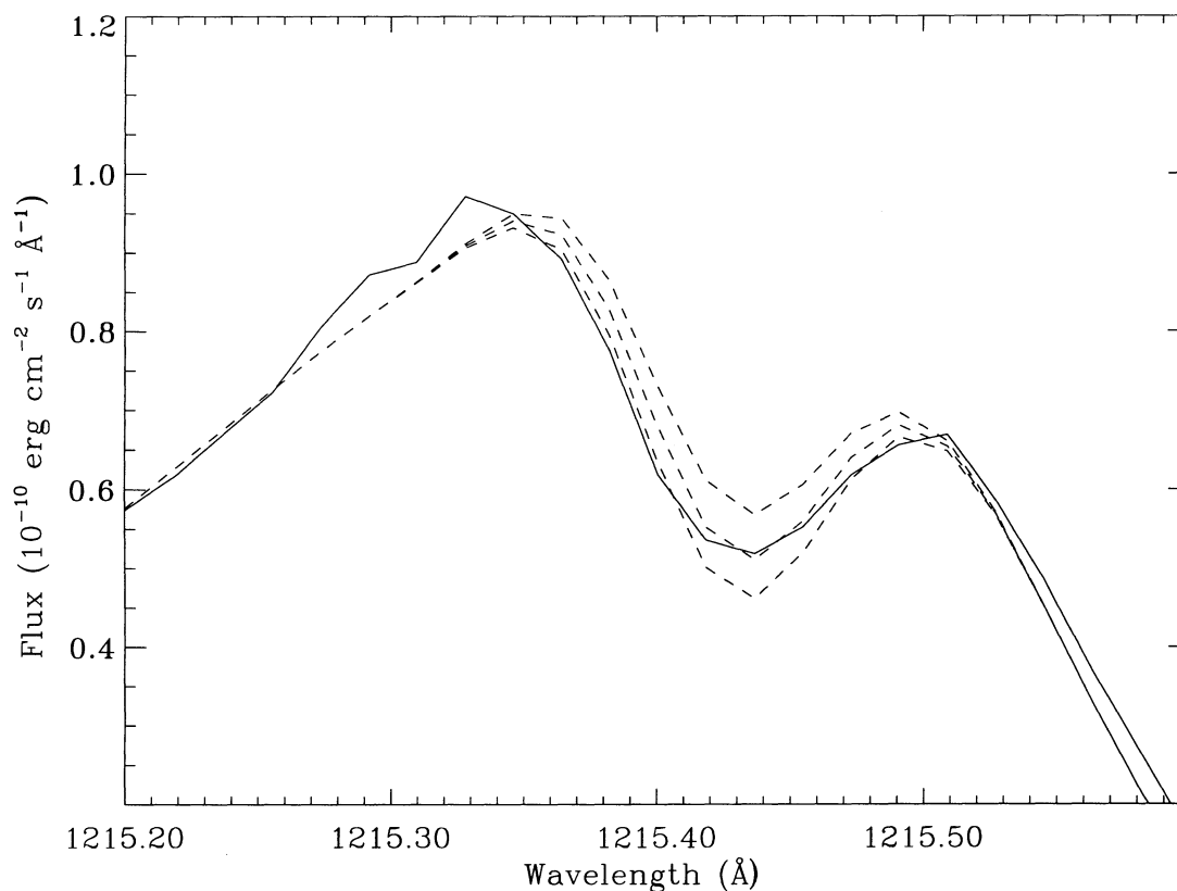
FIG. 13.—Expanded view of the D I line in Procyon's spectrum. Solid line : Observed spectrum. Dashed line : Modified solar profile folded through the two velocity component interstellar medium with the parameters in Table 3 and (from top to bottom) (D/H)_{\text{ISM}} = 1.4, 1.6, \text{ and } 1.8 \times 10^{-5} .
