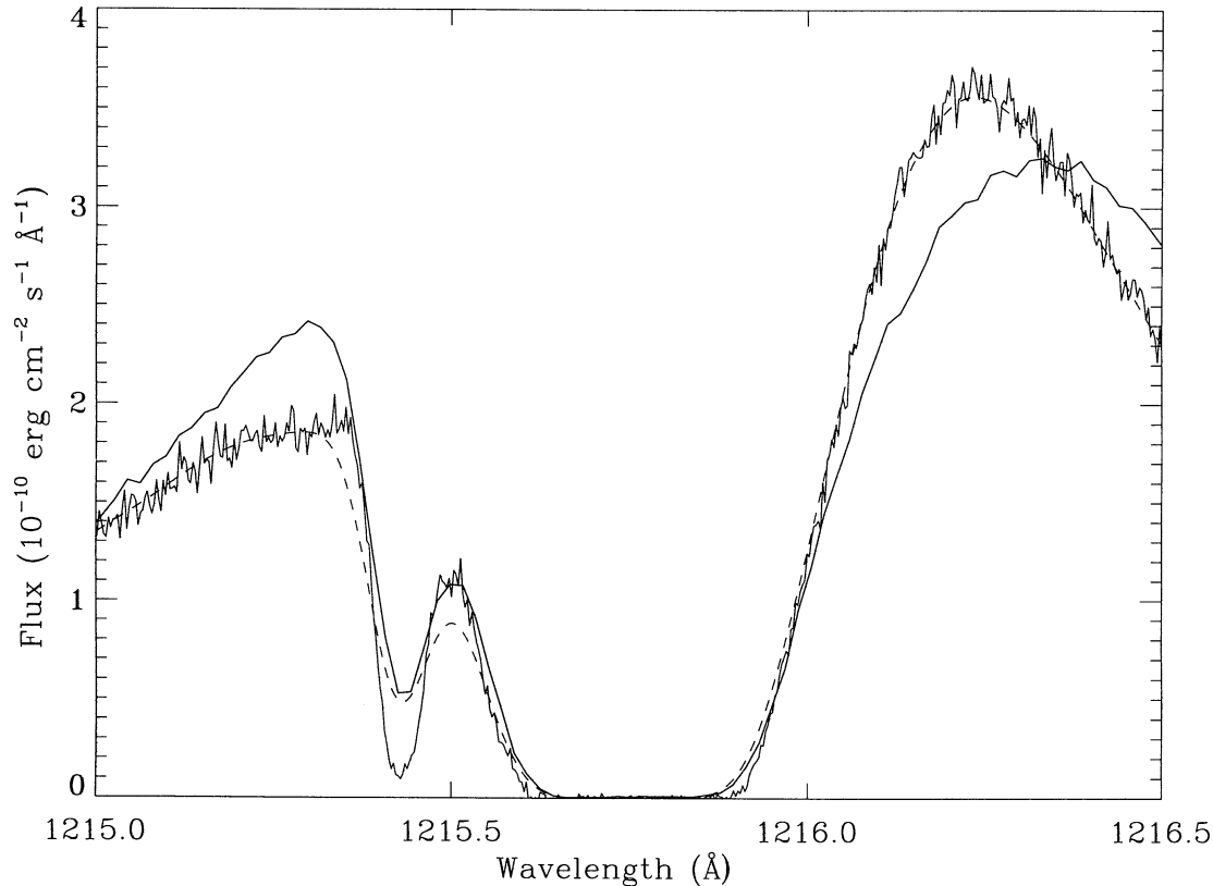
FIG. 1.— \text{Ly}\alpha profiles of Capella at \phi = 0.26 and 0.80 . Irregular solid line , high-dispersion echelle-A spectrum obtained 1991 April 15 at phase \phi = 0.26 . The profile consists of a broad \text{Ly}\alpha emission line produced in the chromospheres of both stars and absorption by interstellar H I and D I ( \Delta\lambda = -0.33 Å relative to hydrogen) along the 12.5 pc line of sight to Capella. Dashed line , \phi = 0.26 spectrum smoothed to the moderate dispersion G160M resolution. Smooth solid line , moderate-dispersion G160M spectrum obtained 1993 September 19 at \phi = 0.80 . The difference between the smoothed \phi = 0.26 spectrum and the \phi = 0.80 spectrum outside of the saturated cores of the H I and D I lines is caused by the different radial velocities of the stellar emission lines at these two phases.
