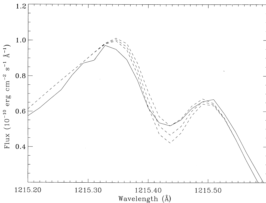
FIG. 11.—Expanded view of the deuterium line in Procyon's spectrum. Solid line : Observed spectrum. Dashed lines : Broadened solar profile folded through the interstellar medium with the parameters in the fourth column of Table 2 and ( top to bottom ) (D/H)_{\text{LISM}} = 1.2, 1.4, \text{ and } 1.6 \times 10^{-5} .
