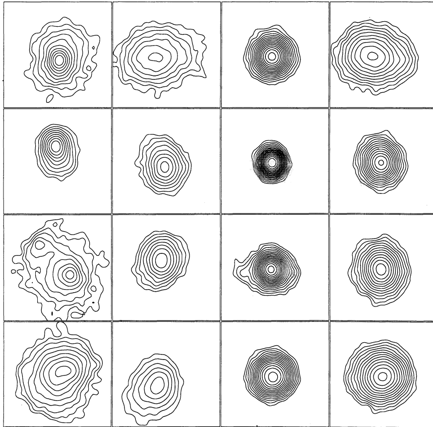
FIG. 5.—Contour maps of Einstein IPC images of four Abell clusters and the artificial IPC images of cluster simulations. From the left to right are: (1) Einstein IPC images, (2) artificial IPC images of \Omega = 1 cluster simulations, (3) artificial images of \Omega_0 = 0.2 simulations, and (4) artificial images of \Omega_0 = 0.2 and \lambda_0 = 0.8 simulations. From top to bottom the clusters are: (1) A496, (2) A644, (3) A1644, and (4) A2256. In producing the artificial IPC images of cluster simulations, we image the simulations at the same redshift as the associated Abell cluster. Contours are spaced by factors of 1.5 in surface brightness. For each image, the surface brightness of the bottom contour is the mean surface brightness in the outermost annulus which satisfies the \langle S/N \rangle > 5 constraint.
