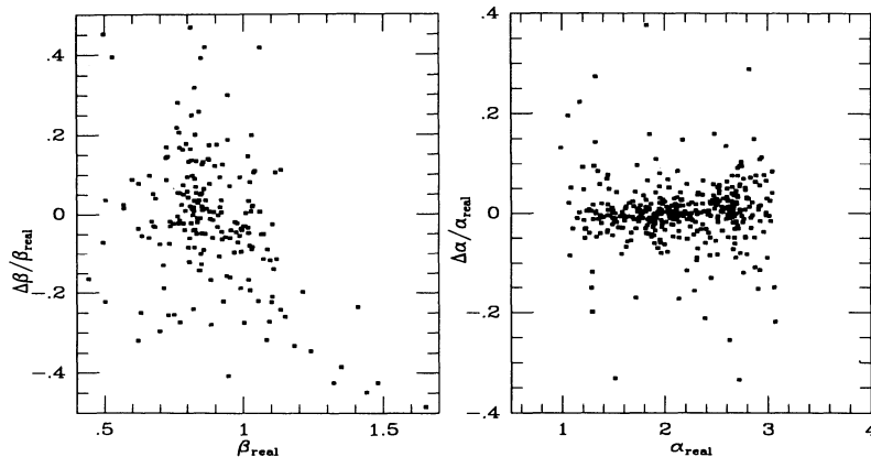
FIG. 4.—Accuracy of two different radial falloff parameters, \alpha and \beta . Left , Fractional error in \beta -measurements as a function of \beta_{\text{real}} ; right , fractional error in the mean falloff \alpha vs. \alpha_{\text{real}} . The width in the \beta -error distribution in \text{rms}_\beta = 17\% , and the bias is \langle \Delta\beta/\beta_{\text{real}} \rangle = -1.6\% . The width in the \alpha -distribution is \text{rms}_\alpha = 7.5\% , and the bias is \langle \Delta\alpha/\alpha_{\text{real}} \rangle = 0.2\% .
