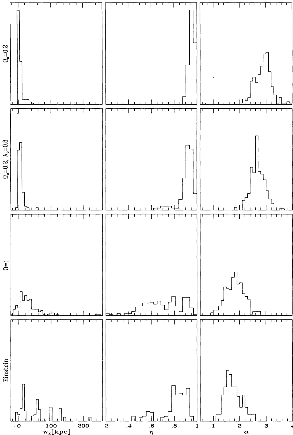
FIG. 6.—Comparing X-ray morphologies. From left to right, each column contains normalized distributions of (1) emission-weighted centroid variation w_x in h_{50}^{-1} kpc, (2) emission-weighted axial ratio \eta , and (3) radial falloff \alpha . From top to bottom, the rows correspond to the following cosmological models: (1) \Omega_0 = 0.2 , (2) \Omega_0 = 0.2 and \lambda_0 = 0.8 , and (3) \Omega = 1 ; the bottom row is the Einstein IPC sample. Table 3 lists the means and widths of these distributions.
