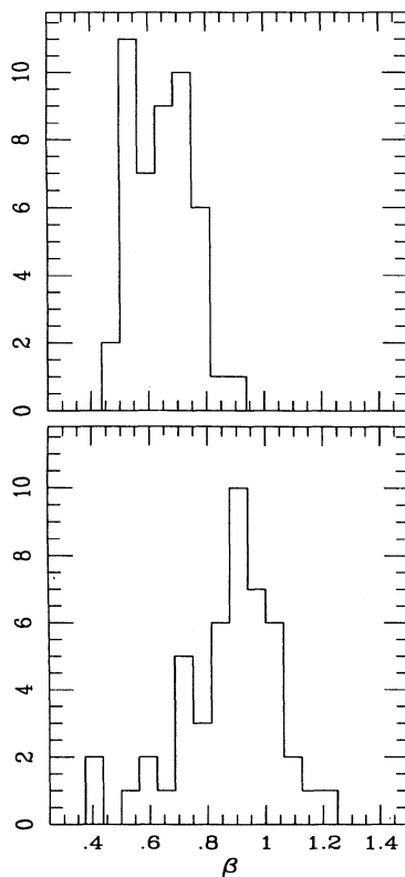
FIG. 7.—We demonstrate the effects of ejection from galaxies on the cluster radial falloff using cluster simulations which include gas ejection (Metzler & Evrard 1994). The histograms contain the results of \beta -fits to idealized images of 47 different clusters. The top histogram is the radial falloff for those clusters evolved with ejection from galaxies ( \langle\beta\rangle = 0.65 ), and the bottom histogram contains the radial falloff for the identical clusters evolved without ejection ( \langle\beta\rangle = 0.87 ).
