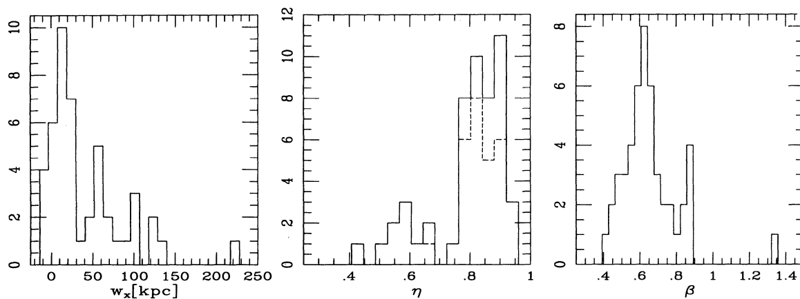
FIG. 3.—X-ray morphologies of observed clusters. From left to right are: (1) distribution of emission-weighted centroid variation w_x in kiloparsecs for a sample of 43 clusters, (2) distribution of emission-weighted axial ratios \eta for a sample of 51 clusters, and (3) distribution of radial falloff \beta for 48 clusters. The mean and root mean square width of the three distributions are (1) \langle w_x \rangle = 41.3 kpc and \text{rms}_w = 47.4 kpc, (2) \langle \eta \rangle = 0.80 and \text{rms}_\eta = 0.12 , and (3) \langle \beta \rangle = 0.65 and \text{rms}_\beta = 0.16 . The dashed line histogram in the \eta -distribution contains 38 clusters. The 13 clusters removed from the original sample have central cooling times significantly less than 10^{10} yr (Edge et al. 1992; Stewart et al. 1984).
