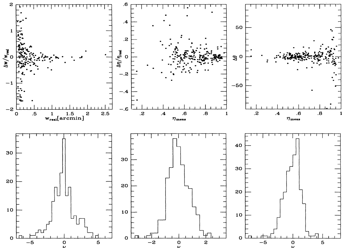
FIG. 2.—Measurement accuracy evaluated using a set of over 200 artificial IPC images. The top row contains (from left to right): (1) fractional error in the centroid variation [ \Delta w/w_{\text{real}} = (w_x - w_{\text{real}})/w_{\text{real}} ] vs. real centroid variation w_{\text{real}} , (2) fractional error in the axial ratio [ \Delta\eta/\eta_{\text{real}} = (\eta_{\text{meas}} - \eta_{\text{real}})/\eta_{\text{real}} ] vs. measured axial ratio \eta_{\text{meas}} , and (3) absolute error in the orientation angle ( \Delta\theta in degrees) vs. measured axial ratio \eta_{\text{meas}} . The mean errors for the three parameters are \langle\Delta w/w_{\text{real}}\rangle = -7.6\% (for all w_{\text{real}} > 0.3 ), \langle\Delta\eta/\eta_{\text{real}}\rangle = -0.7\% , and \langle\Delta\theta\rangle = -0.85 . The bottom row contains the histogram of scaled errors ( \nu = \Delta/\sigma , where \Delta is the error and \sigma is the uncertainty) for each measured parameter. The best Gaussian fits to the \nu -distributions have the widths \sigma_w = 1.34 , \sigma_\eta = 0.73 , and \sigma_\theta = 1.49 . For each parameter we use these widths to correct our uncertainties in order to obtain a \nu -distribution of nominal width.
