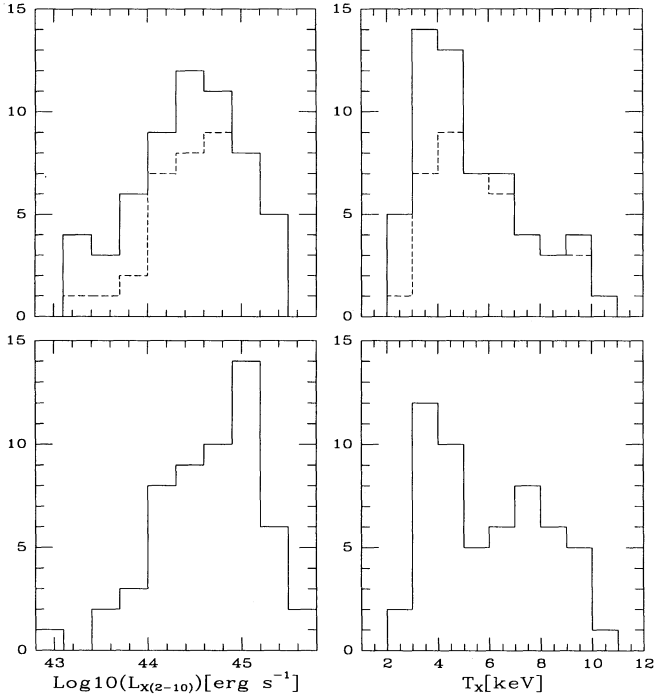
FIG. 1.—Completeness of the Einstein sample. Left-hand column : Distributions of 2–10 keV X-ray luminosity for ( bottom ) the 55 members of the flux-limited Edge et al. (1990) sample and ( top ) the 58 Einstein clusters with published luminosities (Edge et al. 1990; David et al. 1993). The dashed lines in the top plot form the distribution for the 41 of 58 Einstein clusters contained in the Edge et al. flux-limited sample. Right-hand column : Analogous arrangement of the distributions in X-ray temperature. The K-S test demonstrates that there is a reasonable probability that these three samples are drawn from the same parent distribution.
