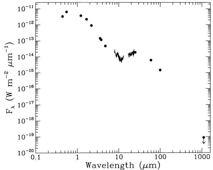
FIG. 2.—Complete SED of SAO 26804. The sources of all the data are listed in Table 1.
