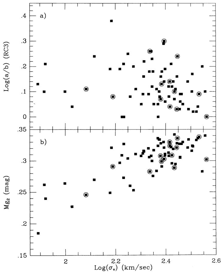
FIG. 7.— \sigma_v vs. (a) a/b , and (b) \text{Mg}_2 for our sample. Symbols as in Fig. 1.
