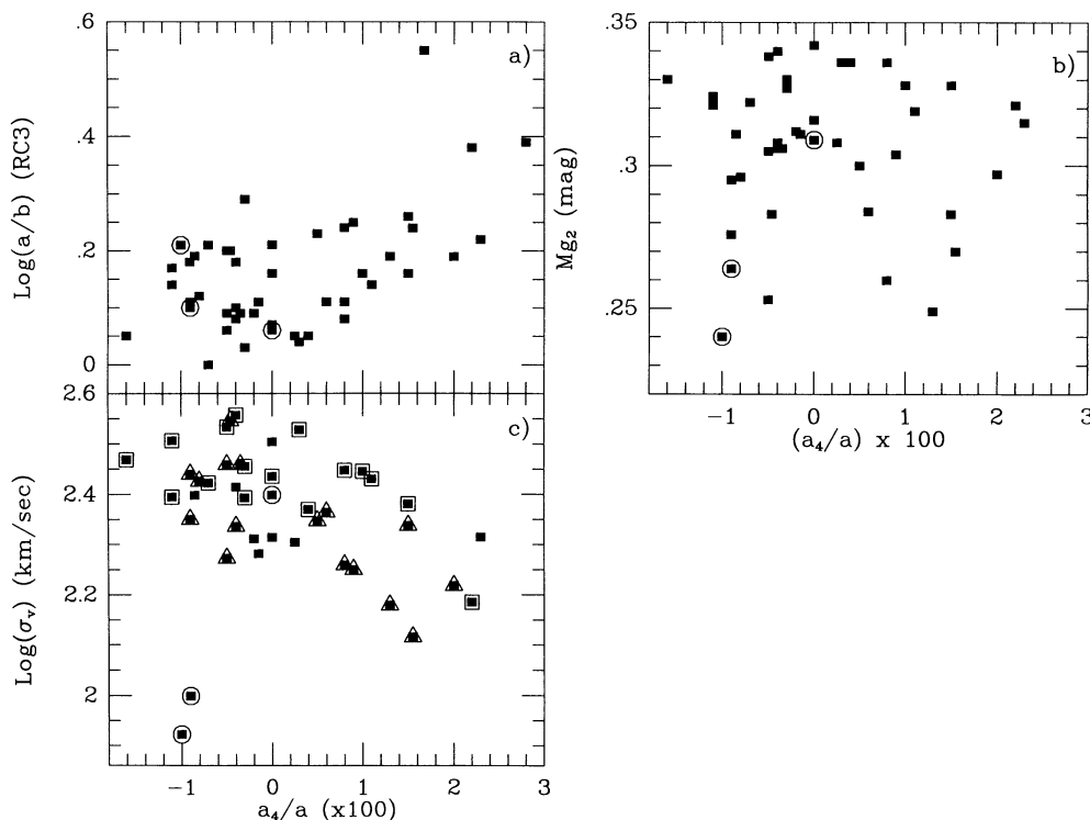
FIG. 9.— a_4 vs. (a) a/b , (b) Mg_2 , and (c) \sigma_v , for our sample. Symbols as in Fig. 8. In (c) the points enclosed in squares are the systems with the highest 40% of Mg_2 values; those enclosed in triangles are the lowest 40%.
