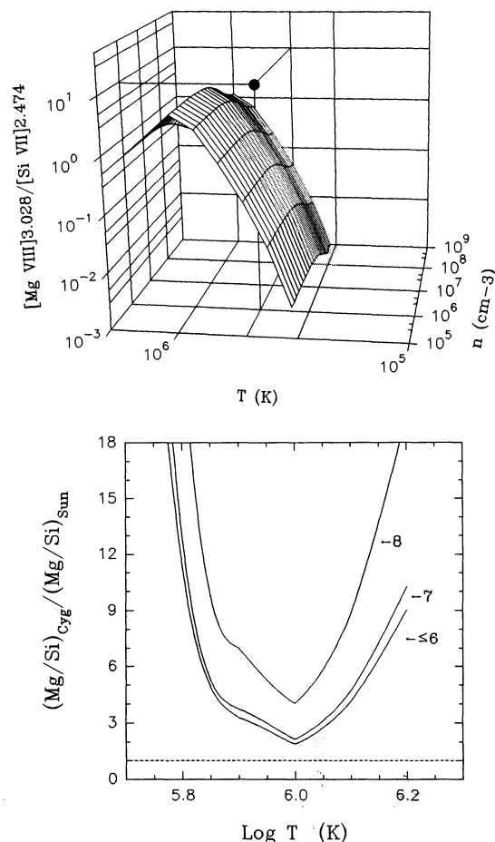
FIG. 14.—Predicted [Mg VIII] 3.028 \mu\text{m} /[Si VII] 2.474 \mu\text{m} line ratio as a function of electron density and ionization temperature, compared with a measured value in V1974 Cyg. The surface shown in the upper panel was calculated using eq. (3) of Greenhouse et al. (1993) and solar photospheric abundances from Grevesse & Anders (1989). Selective extinction between the L- and K-band lines is ignored. The solid data point shown corresponds to a [Mg VIII] 3.028 \mu\text{m} measurement on day 243.4 (see Table 1) and is plotted at our derived density and temperature for this epoch (§ 3.3). The observed ratio lies above the surface, suggesting that V1974 Cyg was overabundant in Mg with respect to Si relative to the solar photosphere. The lower panel shows the gas phase abundance of magnesium relative to silicon as a function of assumed electron density and ionization temperature. The curve labels are values of \log n_e , and the dashed line denotes solar proportions of these elements.
