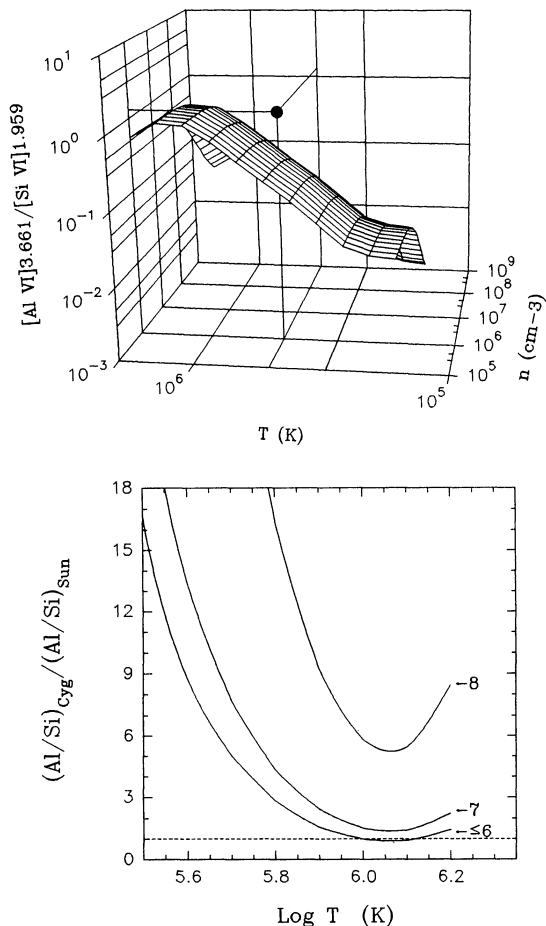
FIG. 13.—Predicted [Al VI] 3.661 \mu\text{m} /[Si VI] 1.959 \mu\text{m} line ratio as a function of electron density and ionization temperature, compared with measured value in V1974 Cyg. The surface shown in the upper panel was calculated using eq. (3) of Greenhouse et al. (1993) and solar photospheric abundances from Grevesse & Anders (1989). Selective extinction between the L- and K-band lines is ignored. The solid data point shown corresponds to a [Al VI] 3.661 \mu\text{m} measurement on day 243.4 (see Table 1) and is plotted at our derived density and temperature for this epoch (§ 3.3). The observed ratio lies above the surface, suggesting that V1974 Cyg was overabundant in Al with respect to Si relative to the solar photosphere. The lower panel shows the gas phase abundance of aluminum relative to silicon as a function of assumed electron density and ionization temperature. The curve labels are values of \log n_e , and the dashed line denotes solar proportions of these elements.
