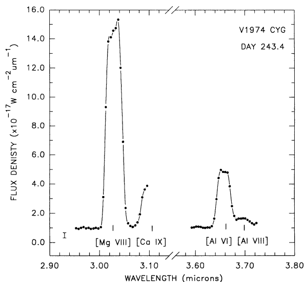
FIG. 11.—High spectral resolution 2.940–3.740 \mu\text{m} composite spectrum (derived from observations at two grating positions) of V1974 Cyg obtained on day 243.4 (1992 October 18.4 UT) from the NASA IRTF 3 m telescope (+CGAS). Prominent spectral features are infrared coronal lines [\text{Mg VIII}] , [\text{Al VI}] , and [\text{Al VIII}] . We interpret the feature at 3.091 \mu\text{m} as the 3s3p^3P_1 \rightarrow 3P_2 transition of [\text{Ca IX}] . The [\text{Mg VIII}] and [\text{Al VI}] lines observed during this epoch are velocity-resolved at 2600 \text{ km s}^{-1} FWHM, indicating that no appreciable deceleration of the ejecta had occurred since the onset of the optically thin emission-line phase (Fig. 1). The increase in the [\text{Al VI}] intensity from day 204.4 (Fig. 10) and the large [\text{Mg VIII}]/[\text{Al VI}] intensity ratio observed on day 243.4 suggest that the coronal line phase was near maximum. A representative 1\sigma error bar is given at the left of each spectral segment, and a cubic spline has been drawn through the data points as a visual aid.
