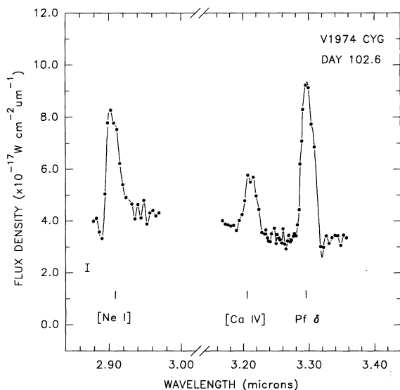
FIG. 6.—High spectral resolution 2.88–3.38 \mu\text{m} composite spectrum (derived from observations at two grating positions) of V1974 Cyg obtained on day 102.6 (1992 May 30.6 UT) from the NASA IRTF 3 m telescope (+CGAS). Prominent spectral features are the Pf \delta hydrogen recombination line, [Ne I], and [Ca IV]. A representative 1\sigma error bar is given at the lower left of the panel, and a cubic spline has been drawn through the data points as a visual aid.
