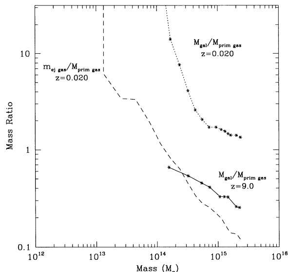
FIG. 6.—Value of three mass ratios plotted against enclosed mass (against radius which encloses that mass): mass in galaxies over mass in (necessarily primordial) gas at z = 9.0 (solid curve); mass in galaxies over mass in primordial gas at z = 0.02 (dotted curve); mass in ejected gas over mass in primordial gas at z = 0.02 (dashed curve).
