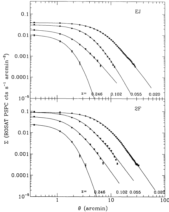
FIG. 11.—Surface brightness profiles for both runs, at the four lowest redshifts imaged in Fig. 10. Also shown are fits to the \beta -model. No data are shown where the surface brightness drops below the fiducial choice for the background of 3 \times 10^{-4} counts \text{s}^{-1} \text{arcmin}^{-2} . Table 4 gives the best-fit parameter values and errors.
