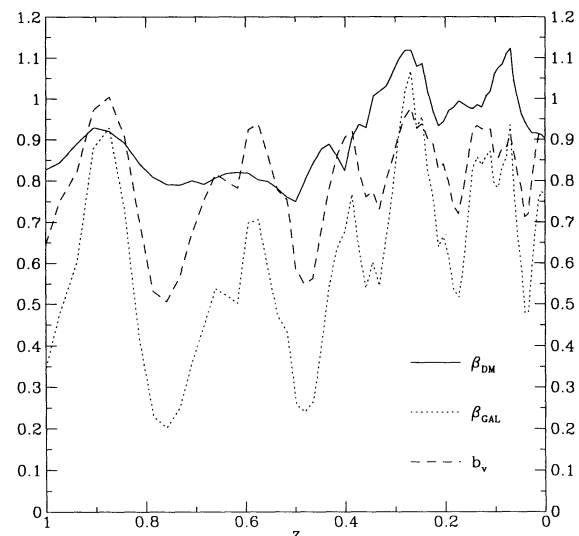
FIG. 14.—Redshift evolution of the true values of \beta , calculated using the mean temperature and one-dimensional velocity dispersion within a comoving radius of 1 Mpc. The solid line shows \beta_{\text{DM}} using the dark matter’s velocity dispersion; the dotted line shows \beta_{\text{gal}} with a one-dimensional velocity dispersion calculated from the galaxies within 1 Mpc. The dashed line shows the velocity bias factor, expressed as the ratio of the two velocity dispersions, b_v = \sigma_{\text{gal}}/\sigma_{\text{DM}} . Some values from this plot are shown in Table 5. A persistent velocity bias is evident which leads to \beta_{\text{gal}} < 1 .
