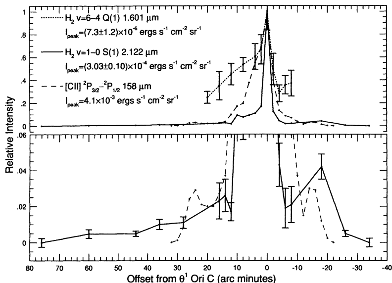
FIG. 1.— Top : Right ascension strip map ( \delta_{1950} = -05^{\circ}25'16'' ) across the face of the Orion molecular cloud in the H 2 v = 6-4 Q(1) and v = 1-0 S(1) lines (49" beam) along with the 158 \mu\text{m} [C II] line (55" beam; Stacey et al. 1993). The [C II] cut is offset \sim 75' to the north of \theta^1 Ori C. We have normalized the line intensities by the peak values shown in the figure and have plotted the v = 6-4 Q(1) data with 1 \sigma error bars. We have not dereddened the H 2 line strengths. Bottom : H 2 v = 1-0 S(1) and [C II] R.A. cuts plotted on a scale suitable to the low-level emission, along with the 1 \sigma error bars for the v = 1-0 S(1) data points.
