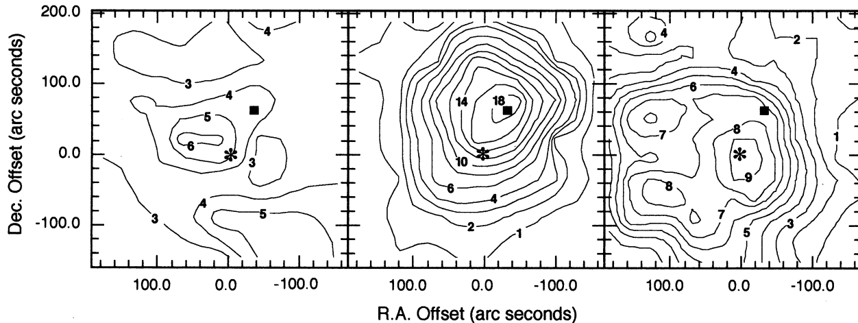
FIG. 2.— Left : v = 6-4 Q(1) map of the Orion H II region/molecular cloud interface. The peak contour level corresponds to a surface brightness of 6.4 \times 10^{-6} ergs s^{-1} cm^{-2} sr^{-1} in a 65'' beam. The 0, 0 position is at \theta^1 Ori C. We have marked \theta^1 Ori C and the BN-KL outflow by an asterisk and a square, respectively. Center : H_2 v = 1-0 S(1) map of the interface region. The contour units are in multiples of the lowest contour level, which corresponds to a surface brightness of 3.53 \times 10^{-5} ergs s^{-1} cm^{-2} sr^{-1} in a 150'' beam. Right : 158 \mu m [C II] map of Stacey et al. 1993 ( 55'' beam). The contour units are in multiples of the lowest contour level ( 3.9 \times 10^{-4} ergs s^{-1} cm^{-2} sr^{-1} ).
