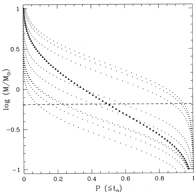
FIG. 2.—Distribution of P_k(\leq t_0) values is shown with dots for all nine OGLE lensing events for a series of models with various values of the lens masses, \log M , with all lenses having the same mass in a given model. The average value of the probability \langle P \rangle is shown for every model with a filled triangle. For the correct model the values of P_k should be randomly distributed in the interval (0, 1), and it should have \langle P \rangle = 0.5 . This model is shown with a dashed horizontal line corresponding to M/M_\odot = 0.65 . The “full disk” with \rho_0 = 0.415 M_\odot \text{ pc}^{-3} plus the KP bulge contributed to the lensing.
