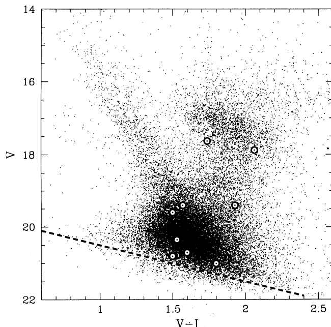
FIG. 1.—Locations of the nine OGLE lensing events (larger circles) are shown in the color-magnitude diagram for Baade's window and the Galactic bar fields combined. Only \sim 5\% of all OGLE stars are shown. The dashed line shows the limit of lens detectability given by the condition I < 19.5 .
