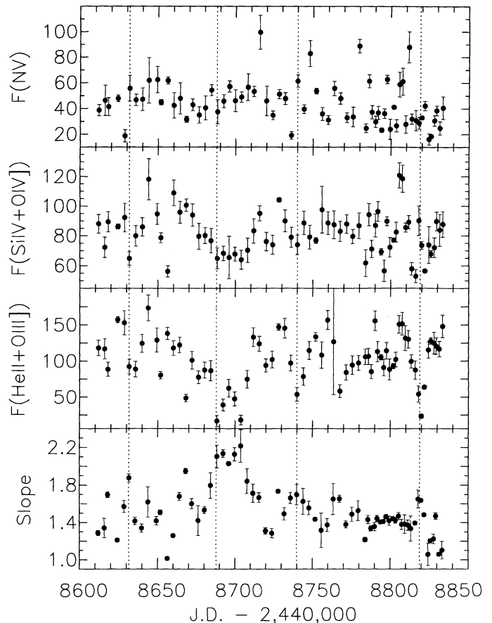
FIG. 4.—Light curves for N v \lambda 1240 (top), Si IV + O IV] \lambda 1402 (upper middle), and He II \lambda 1640 + O III] \lambda 1663 (lower middle) fluxes, and frequency spectral index \alpha_v (bottom). All quantities were derived from the GEX plus spectral fitting method. Fluxes are in units of 10^{-14} ergs \text{cm}^{-2} \text{s}^{-1} . Dashed vertical lines have been drawn to facilitate comparisons with Figs. 2 and 3.
