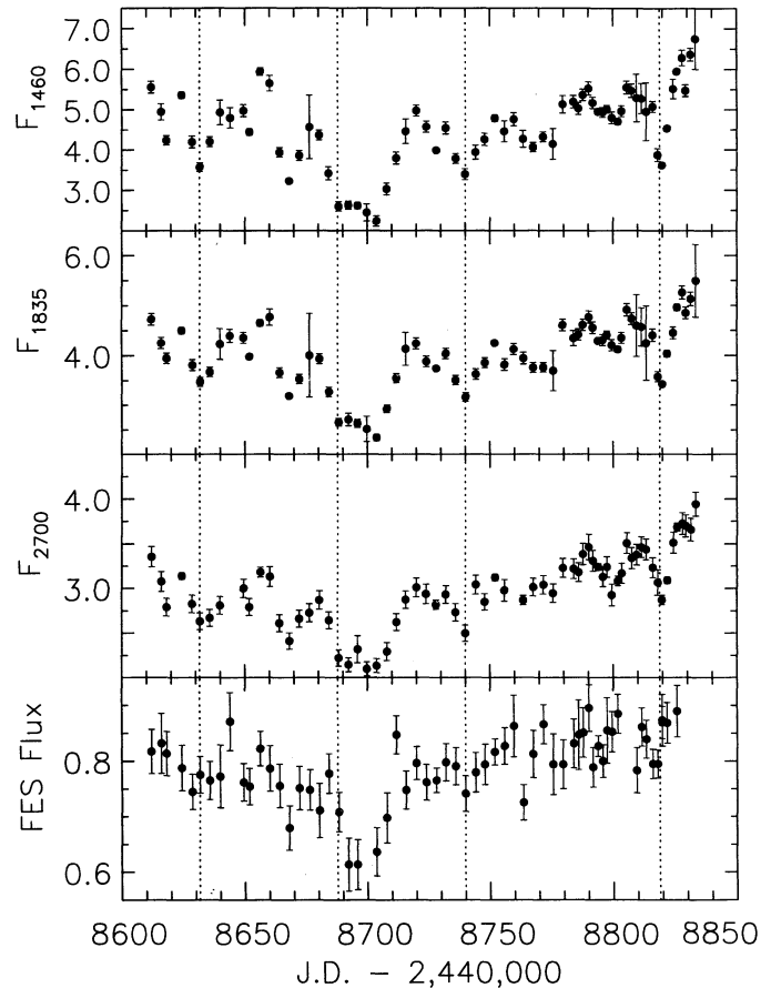
FIG. 2.—Light curves for F_{1460} (top), F_{1835} (upper middle), and integrated F_{2700} (lower middle), and relative FES fluxes (bottom). All UV fluxes are in units of 10^{14} erg \text{cm}^{-2} \text{s}^{-1} Å ^{-1} and were derived from the GEX plus spectral fitting method. The FES fluxes are as defined in eq. (3). Dashed vertical lines have been drawn to facilitate comparisons with Figs. 3 and 4.
