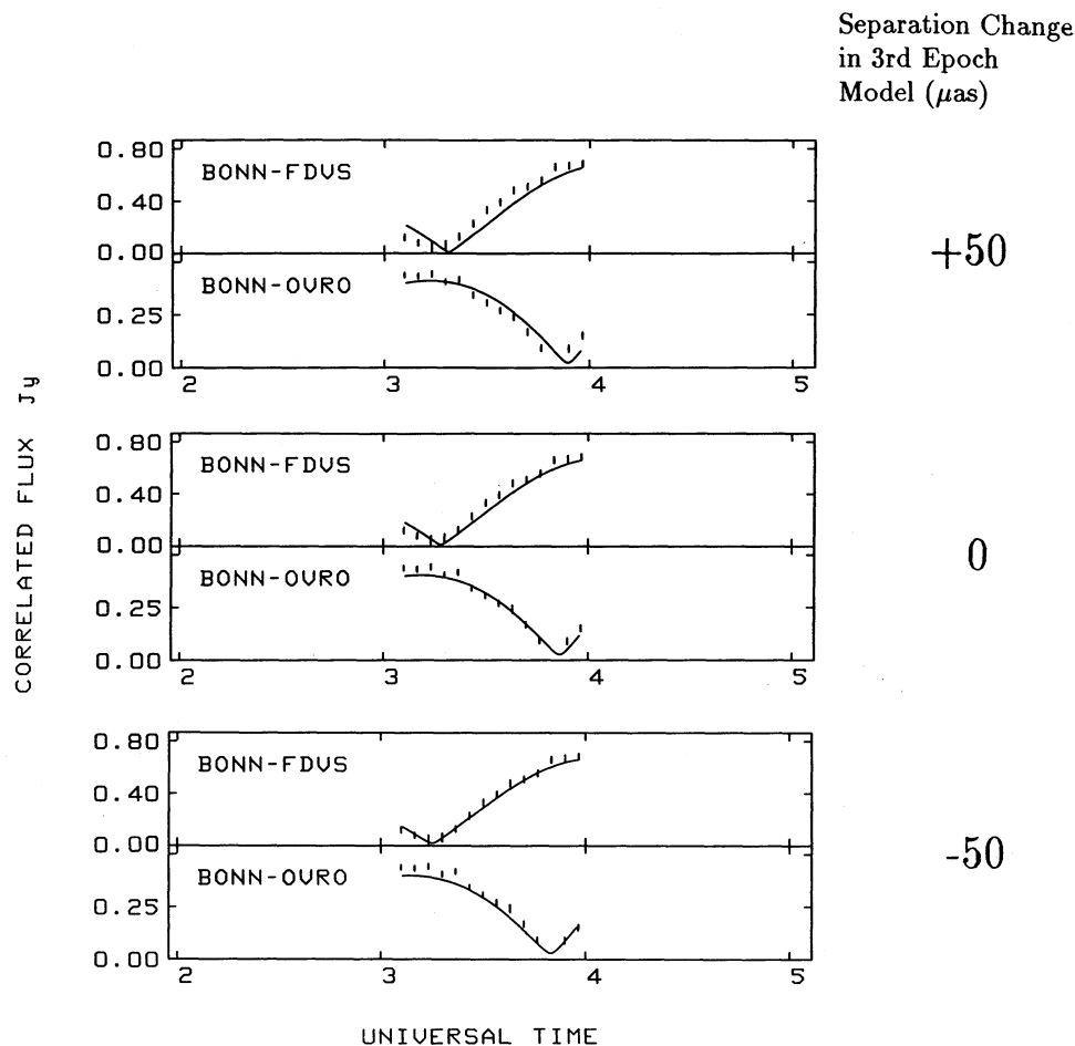
FIG. 2.—Illustration of a possible change in 0108+388 between epochs 2 and 3. Middle panel shows fit of third-epoch model to second-epoch data. Top and bottom panels show the fit of versions of the third-epoch model in which the separation of the two main components is respectively increased and decreased by 50 \mu\text{as} . Note that the goodness of fit is asymmetric with respect to changes in separation, with the best fit occurring for a change of between 0 and -50 \mu\text{as} , corresponding to an increase in component separation between epoch 2 and epoch 3.
