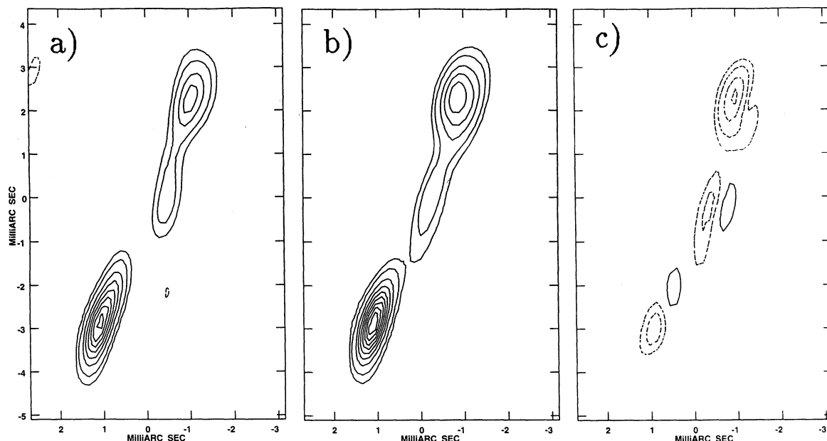
FIG. 4.—Difference between 0711 + 356 images at the two 10.7 GHz epochs. The images are registered on the southern component. In all cases the CLEAN beam has FWHM 1.2 \times 0.4 \text{ mas} in P.A. -15^\circ . Contour levels are at -60, -40, -20, -10, 10, 20, 40, 60, 80, 100, 120, 140 , and 160 \text{ mJy beam}^{-1} . (a) 1984 image. (b) 1981 image. (c) Difference between 1984 and 1981 images.
