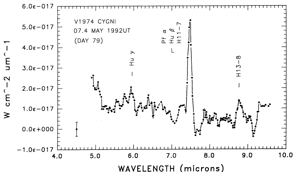
FIG. 1.—The 5–10 \mu\text{m} spectrum of V1974 Cyg obtained on 1992 May 7.4 UT (day 79) from the KAO. Prominent in the spectra are hydrogen recombination lines. A representative mean 1\sigma error bar is given in the lower left of the panel.
