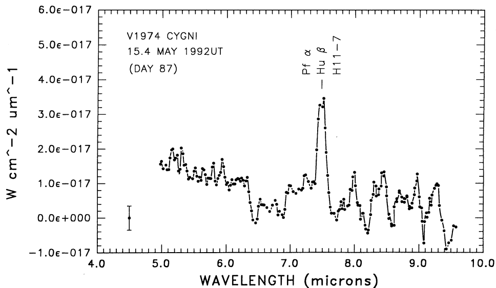
FIG. 2.—The 5–10 \mu\text{m} spectrum of V1974 Cyg obtained on 1992 May 15.4 UT (day 87) from the KAO. The spectrum is still dominated by hydrogen recombination lines. A representative mean 1\sigma error bar is given in the lower left of the panel.
