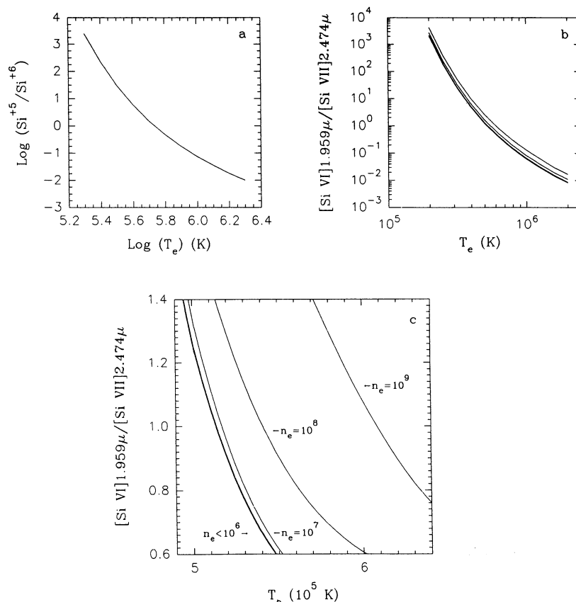
FIG. 6.—The coronal ionization equilibrium of \text{Si}^{+5} and \text{Si}^{+6} as a function of (a) temperature, and (b) and (c) corresponding [Si vi] 1.959 \mu\text{m} /[Si vii] 2.474 \mu\text{m} line intensity ratio at several densities. Fig. 6a is independent of density. Densities in Figs. 6b and 6c are shown in units of \text{cm}^{-3} . Further details are discussed in § 3.1.
