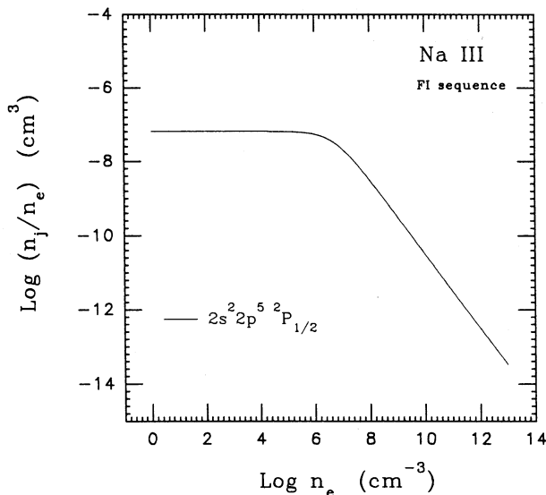
FIG. 8.—Level populations n_j \equiv n(\text{Na}_j^{+2})/n(\text{Na}_{\text{tot}}^{+2}) as a function of electron density n_e . The critical density for collisional deexcitation of the indicated level occurs at the knee of the curve (see Table 2).
