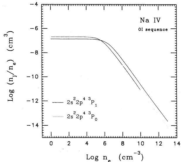
FIG. 9.—Level populations n_j \equiv n(\text{Na}_j^{+3})/n(\text{Na}_{\text{tot}}^{+3}) as a function of electron density n_e . The critical density for collisional deexcitation of the indicated level occurs at the knee of the curve (see Table 2).
