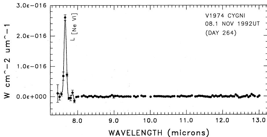
FIG. 5.—The 7–13 \mu\text{m} spectrum of V1974 Cyg obtained on 1992 November 8.1 UT (day 264) from the NASA 1.52 m infrared telescope facility on Mount Lemmon, AZ. A strong [Ne VI] emission line dominates the emergent spectra. A representative mean 1\sigma error bar is given in the lower left of the panel.
