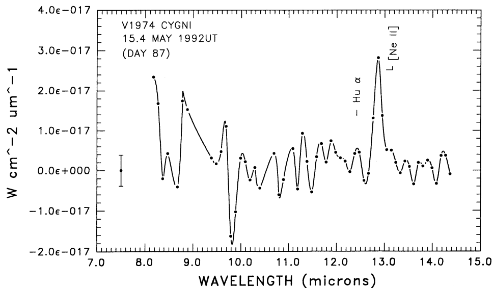
FIG. 3.—The low-resolution 7–14 \mu\text{m} spectrum of V1974 Cyg obtained on 1992 May 15.4 UT (day 87) from the KAO. Emission from [Ne II] is clearly evident. A representative mean 1\sigma bar is given in the lower left of the panel.
