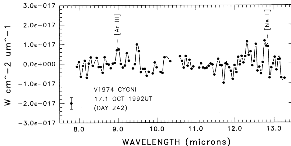
FIG. 4.—The 8–13 \mu\text{m} spectrum of V1974 Cyg obtained on 1992 October 17.1 UT (day 242) from the NASA 1.52 m infrared telescope facility on Mount Lemmon, AZ. Emission lines of [Ar III] and [Ne II] are evident in the spectrum. A representative mean 1\sigma error bar is given in the lower left of the panel. The gap in the spectrum near 10.5 \mu\text{m} is due to a noise spike.
