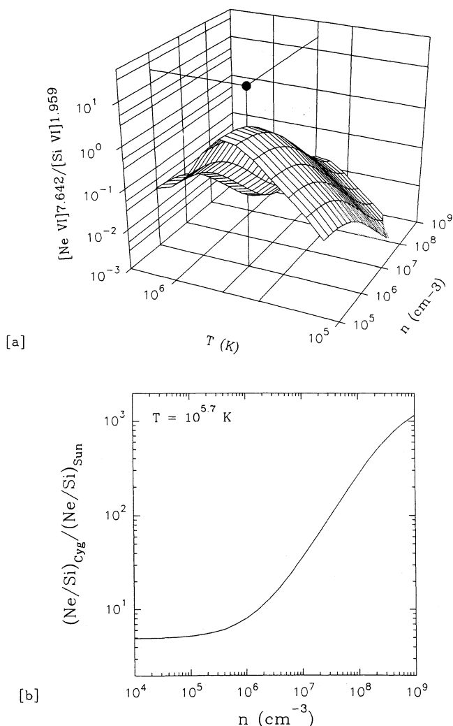
FIG. 7.—(a) The calculated [\text{Ne VI}] 7.642 \mu\text{m}/[\text{Si VI}] 1.959 \mu\text{m} intensity ratio of V1974 Cyg (§ 3.1, eq. [3]) is shown as a function of ionization temperature and electron density for solar photospheric abundances of Ne and Si. The day 264 measured line ratio is plotted as a solid dot. All axes are logarithmic. (b) The derived overabundance of Ne/Si as a function of assumed electron density. We find that at any reasonable density and temperature, a factor of \approx 10 overabundance of neon with respect to silicon is required to account for the observed ratio. Further details are discussed in § 3.1.
