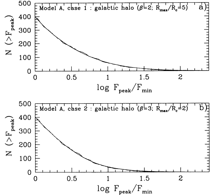
FIG. 3.—A randomly generated sample (400 bursts) of the two cases of model A (a simple Galactic halo distribution). The solid lines indicate the best-fit model A function to each sample (see § 4). The best-fit parameters of model A ( \beta and R_{\text{max}}/R_c ) for these samples are 2.04 and 4.51 (case 1) and 3.08 and 1.92 (case 2). Notice that we use a linear scale (rather than the traditional log scale) on the y-axis because the K-S d measures a linear distance; therefore, with this representation, it is easier to see the deviations of each sample from the best-fit theoretical curve.
