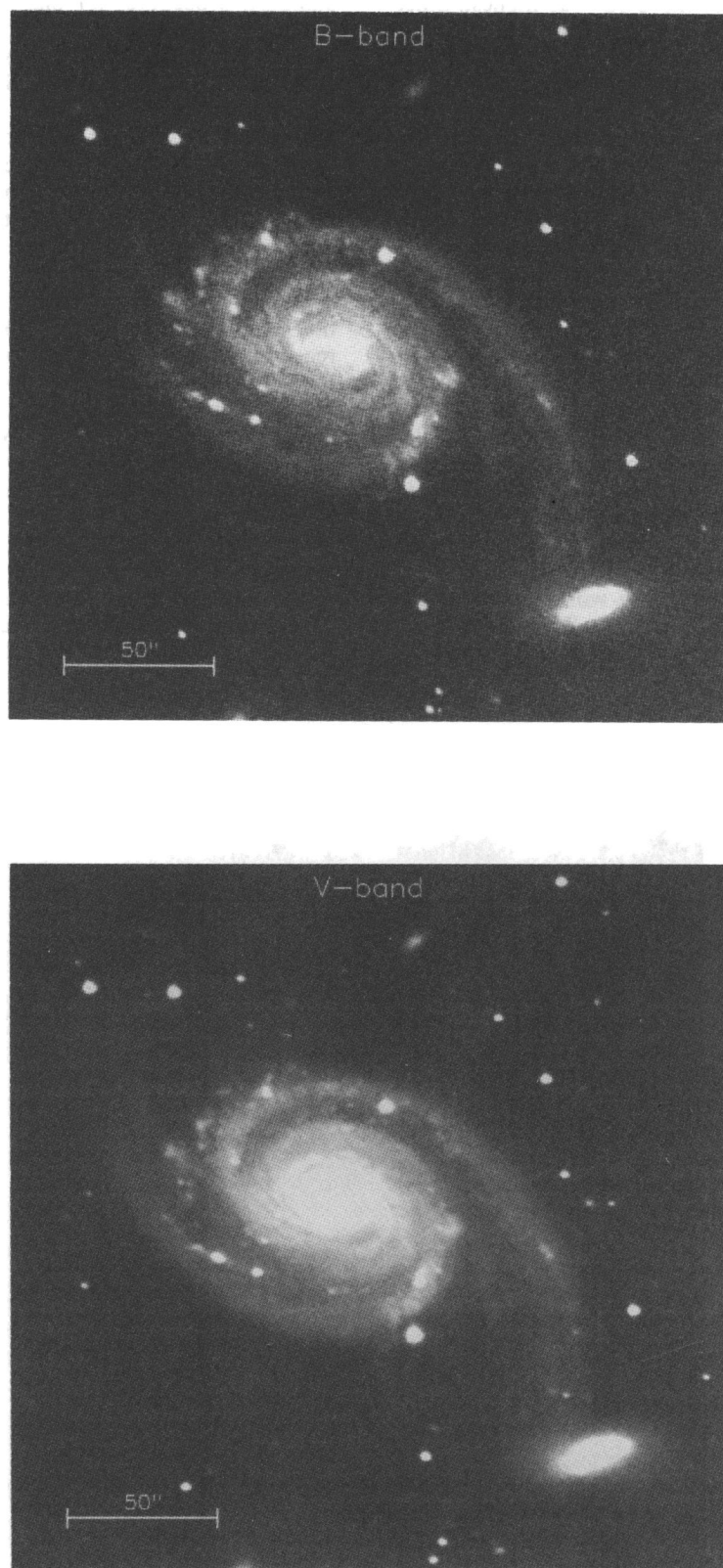
FIG. 2.—Cleaned B , V , R , and I images obtained in Calar Alto
