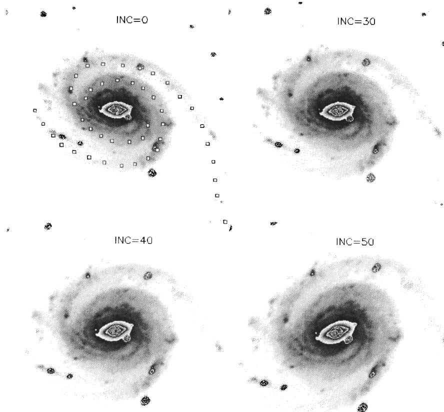
FIG. 4.—Deprojected V image of NGC 7753 for inclinations i = 0^\circ, 30^\circ, 40^\circ, 50^\circ , and position angle P.A. = 53^\circ . The open squares trace the main observed spiral arms.
