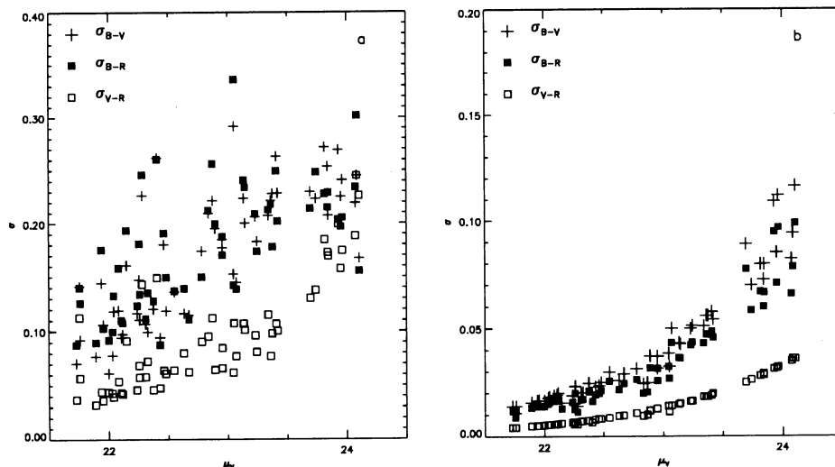
FIG. 10.—Error estimates for color measurements. (a) Standard deviations of the mean colors are shown as a function of the surface brightness in the V band. (b) Poisson noise is displayed in the same measured positions.
