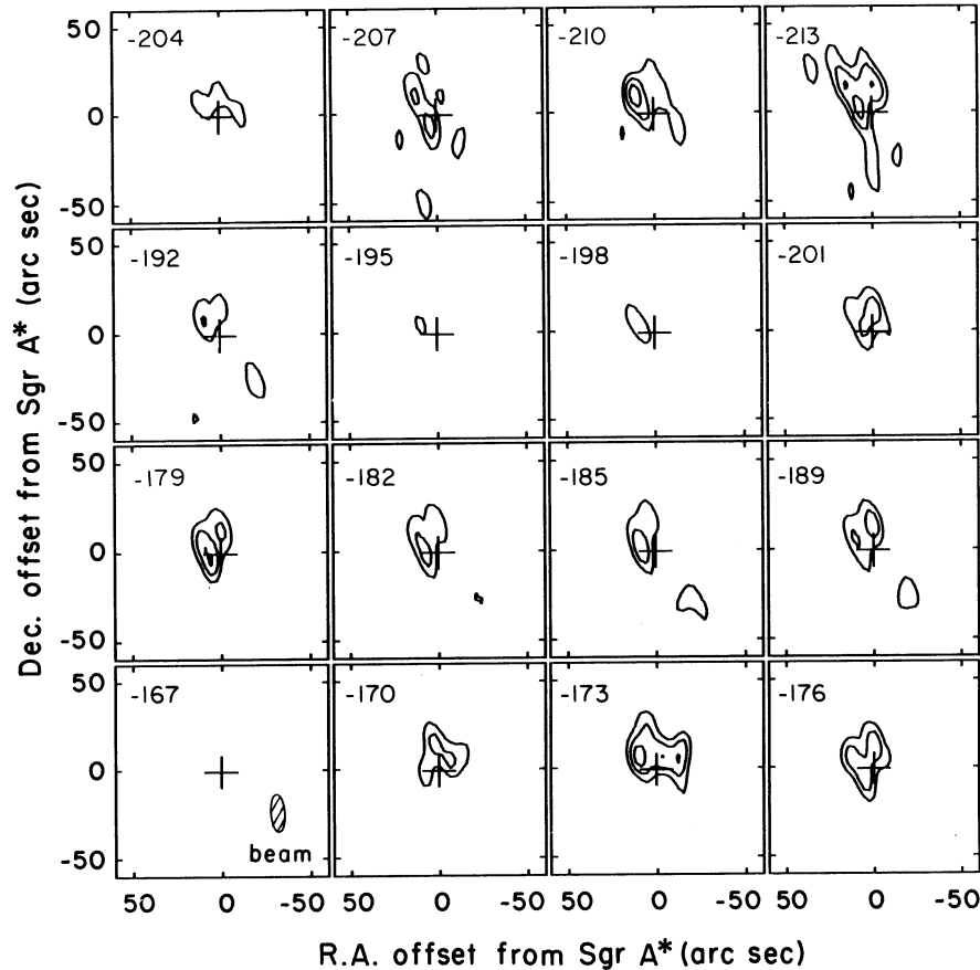
FIG. 3.—Individual channel maps of \text{H}_2\text{CO} absorption for velocities from -167 to -213 \text{ km s}^{-1} . Note that the absorption is located primarily east and northeast of Sgr A* (denoted by the cross). The synthesized beam is shown as an ellipse in the channel at -167 \text{ km s}^{-1} . Contour levels are -20 , -30 , and -40 \text{ mJy beam}^{-1} .
