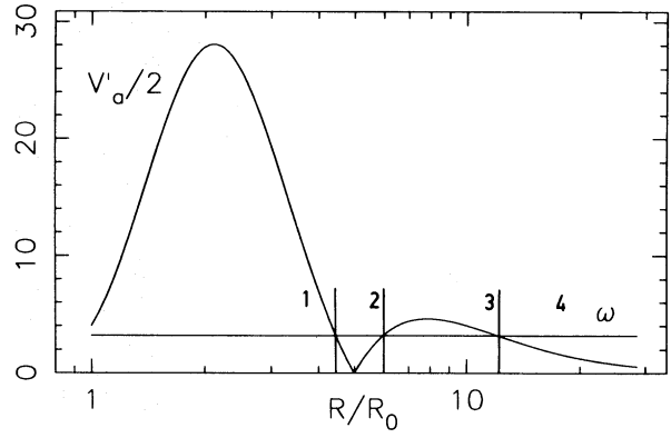
Fig. 4. The profile of the Alfvén speed derivative for the spherically symmetric isothermal atmospheres of Figs. 1 and 2, showing regions of evanescence, (1, 3) and propagation (2, 4), for a given frequency (denoted by the straight line)
