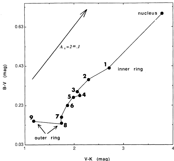
FIG. 3.—A color-color ( B-V , V-K ) plot for each annulus shown in Fig. 1a. This figure illustrates the radial dependence of the color within the disk. The data have been corrected for Galactic interstellar reddening but have not been corrected for internal extinction. The arrow indicates the effect of using A_v = 2^m1 , which was derived for knots 3 and 5 (FH).
