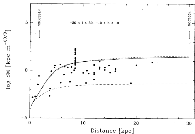
FIG. 4.—Plot of scattering measure against distance from the Sun. The plotted points represent data presented in Tables 2 and 3 and data compiled by Cordes et al. (1991a) that include pulsar measurements and data on scattered AGNs from Fey et al. (1991). AGNs are plotted arbitrarily at a “distance” of 30 kpc. The solid line represents SM calculated from the model of Cordes et al. for l = 0 , b = 0 ; the dotted line corresponds to |l| = 15^\circ , b = 0 ; the dashed line corresponds to l = 0 , |b| = 5^\circ .
