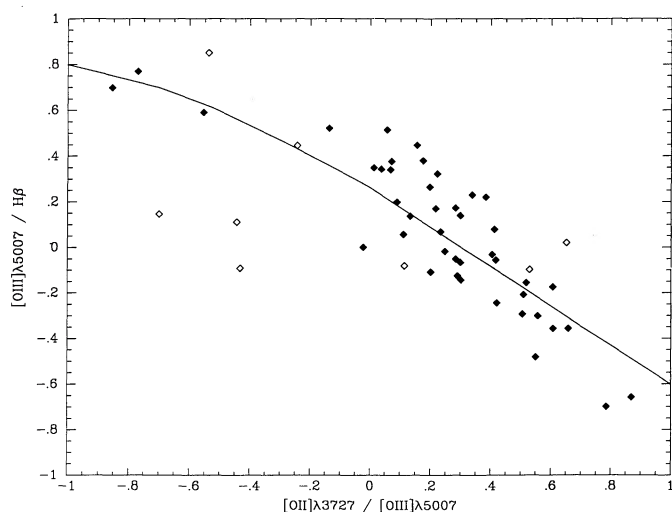
FIG. 7.—Diagnostic diagram for the integrated oxygen emission-line fluxes, following the convention of Baldwin, Phillips, & Terlevich (1981). Solid points denote galaxies dominated by disk emission, and open symbols indicate galaxies with emission dominated by a nonthermal nucleus. The line shows the mean relation for H II regions in the Baldwin et al. study. The [\text{O III}]/\text{H}\beta ratios have been corrected for stellar Balmer absorption. The data shown here have not been corrected for reddening, so most points lie farther to the right than indicated here.
