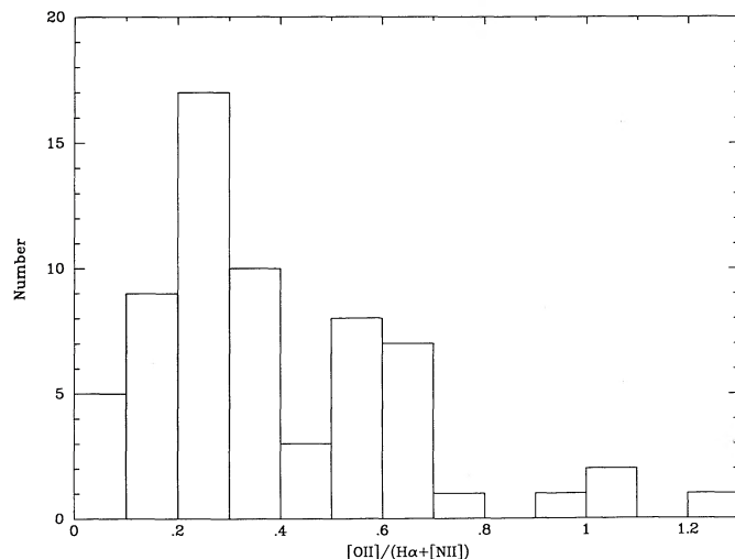
FIG. 12.—Distribution of the ratio of flux in the [O II] \lambda 3727 and H \alpha + [N II] emission lines for this sample. Values are not corrected for reddening or stellar absorption at H \alpha .
