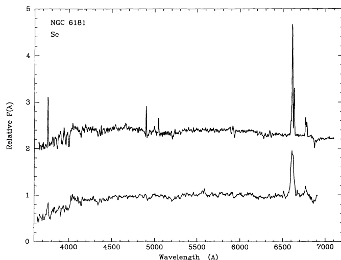
FIG. 1.—Comparison of two spectra of NGC 6181, showing the effects of resolution and spatial sampling. The top spectrum was obtained by drift-scanning a narrow slit over a 90'' \times 60'' region. Resolution is 5–7 Å. The bottom spectrum is a single pointed observation of the central 45'' , with roughly 20 Å resolution.
