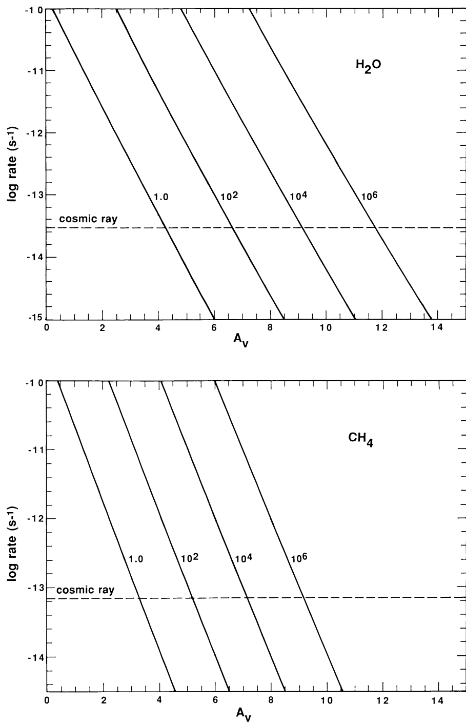
FIG. 3.—The photodestruction rates of \text{H}_2\text{O} , \text{CH}_4 , \text{NH}_3 , and \text{C}_2\text{H}_2 as functions of A_v for 1.0, 10^2 , 10^4 , and 10^6 times the standard interstellar radiation field.
