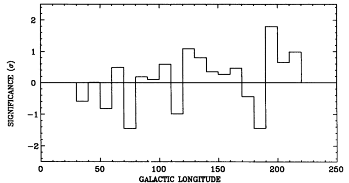
FIG. 6.—Significance of observed number of muon-poor showers with respect to the expected number along the Galactic plane ( |b^{\text{II}}| < 10^\circ ). The bin size is \Delta l^{\text{II}} = 10^\circ . The significance is expressed in units of Gaussian standard deviation \sigma , calculated as in Li & Ma (1983).
