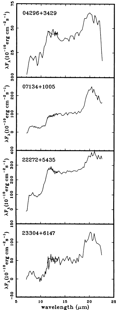
FIG. 1.—LRS spectra of 04296+3429, 07134+1005, 22272+5435, and 23304+6147. In each case, a linear baseline has been removed. The second band has also been shifted to ensure matching with the first band in the overlapping wavelength regions. The spectrum of 04296+3429 has been smoothed over three channels.
