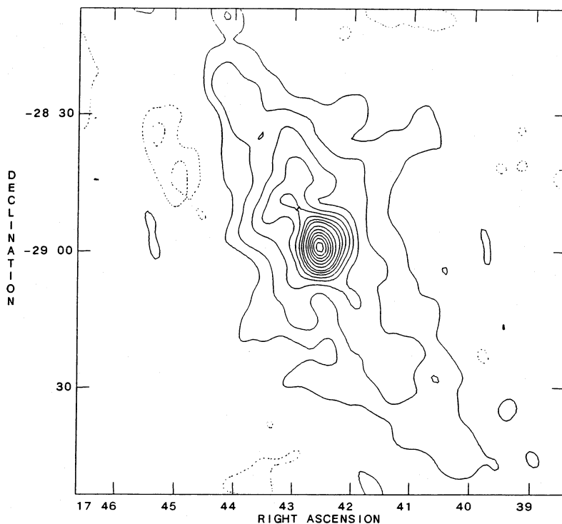
FIG. 1.—Continuum map of the Galactic center region at 327 MHz. The beam size is 5.6' \times 3.4' . The contour levels are -10, -6, -4, -2, 2, 4, 6, 10, 14, 20, 30, 40, 60, 80, 140, and 180 Jy per beam.
