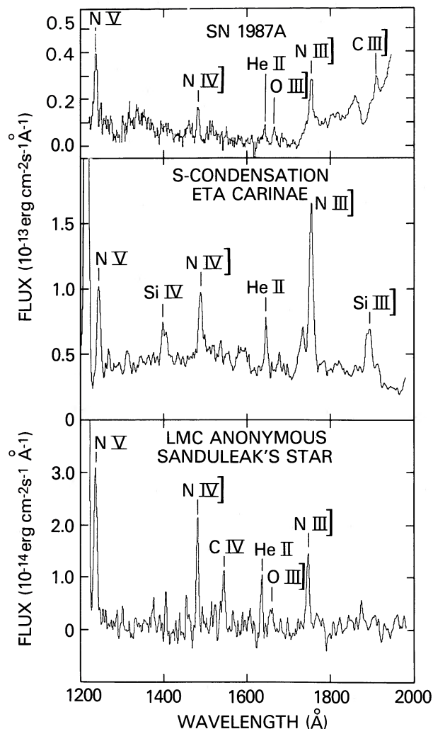
FIG. 1.— Top : IUE low-resolution spectrum in the SWP \lambda\lambda 1200–2000 Å camera of SN 1987A obtained by Fransson et al. (1988), representative of the narrow–low velocity emission spectrum associated with circumstellar material in 1987 December. The spectrum is an average of exposures in which the contributions from several B stars in the aperture have been removed. Narrow emission lines consisting of N v, N iv], He II, O iii], N iii], and C iii] are evident. An E(B-V) = 0.2 has been applied to the spectrum using the LMC extinction values of Fitzpatrick (1986). Middle : The S-Condensation of \eta Carinae obtained by Davidson et al. (1986). The spectrum is not dereddened, but the extinction estimated for the S Condensation is E(B-V) = 0.6 (Davidson et al. 1986). Prominent emission lines of N v, N iv], N iii] are present, together with He II, Si iv], and Si iii] are prominent. Bottom : Low-resolution spectrum obtained on 1985 July 1 (SWP 26732) of LMC Anomalous (Sanduleak's Star) by Kafatos et al. (1983). The relative emission line intensities of N v, N iv], He II, and N iii] are similar to the S-condensation in \eta -Carinae. Weak C iv \lambda\lambda 1548, 1550 emission is present, which may be variable on time scales of at least 3 yr. The intersystem emission lines of C iii] \lambda\lambda 1970, 1909 are not evident, further indicating a depletion of carbon in circumstellar material. The spectrum has not been corrected for reddening.
