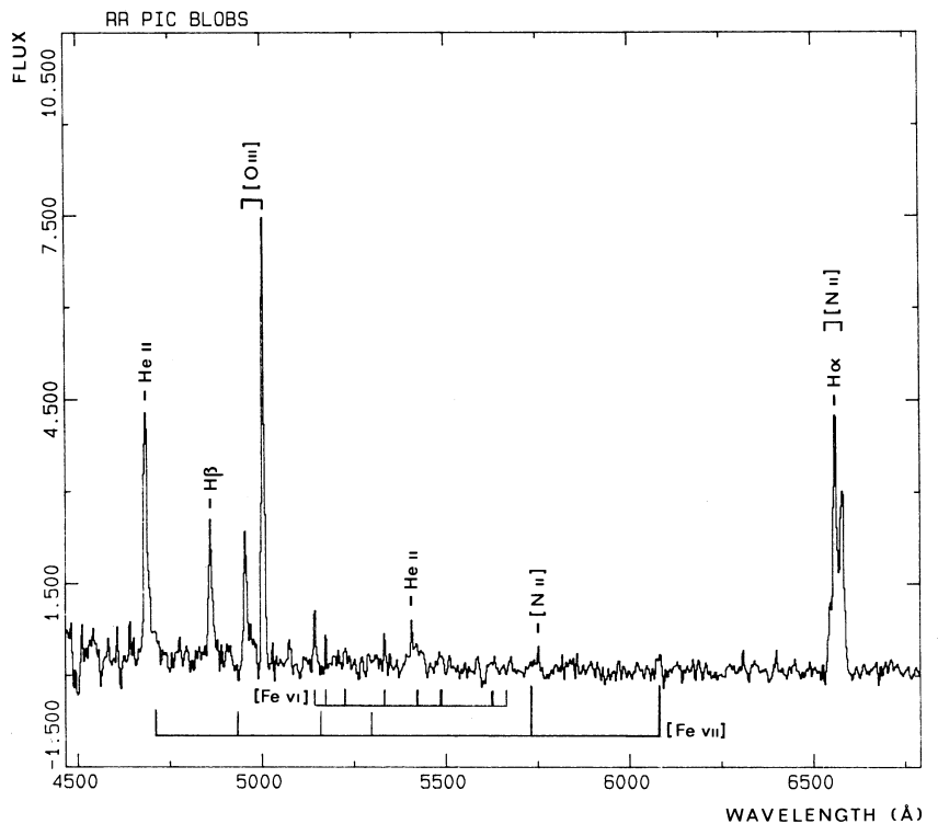
Figure 5: The spectrum of the "polar blobs" of nova RR Pic.
