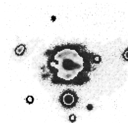
Figure 2: The shells surrounding the recurrent nova T Pyx, taken through an H \alpha filter. For this composite, the central section of the highly amplified picture was set to zero, then a lower amplification image of the well-known central nebula was inserted.
