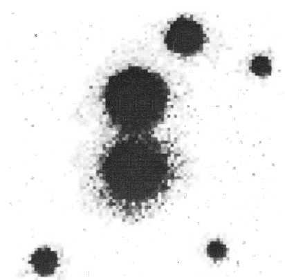
Figure 1: The shell surrounding nova BT Mon, taken through an H \alpha filter.
