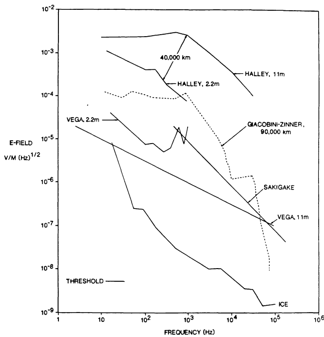
Fig. 8. Plasma wave spectra from Halley (Vega-1 and -2) and Giacobini-Zinner (ICE), together with E-field threshold curves for the comet plasma wave instruments
