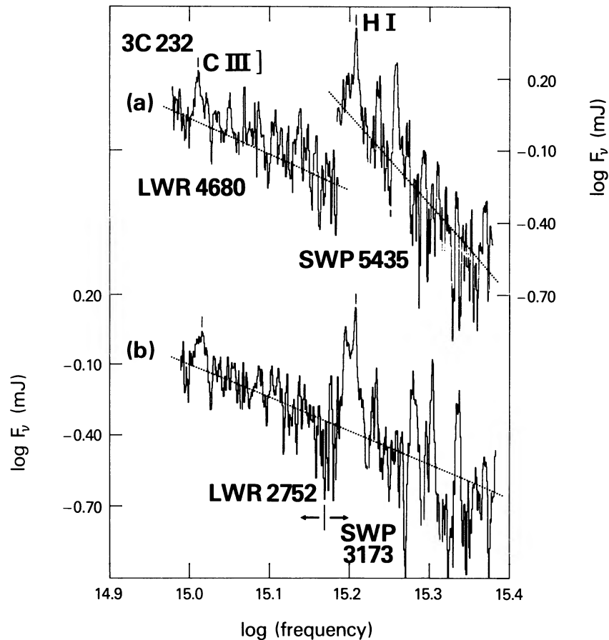
FIG. 2.—Flux distributions for 3C 232. The images SWP 3173 and LWR 2752 were acquired on days 300 and 302 in 1978, while SWP 5435 and LWR 4680 were obtained on days 153 and 154 in 1979. Approximate power-law fits were made to the data sets from both IUE cameras. These fits are represented by dotted lines. The features C III] 1909 Å and H I–Ly \alpha are also denoted. These data clearly indicate that the flux near H I–Ly \alpha has decreased by a factor of 2 between the acquisition of SWP 5435 and LWR 4680, roughly 24 hr later. The data for image LWR 4680 also show a much shallower power-law slope than do those for SWP 5435. The data for SWP 3173 and LWR 2752 show no hint of flux variation between the two exposures. The false “comet” feature corresponding to 940 Å in SWP 3173 (See Fig. 1 and text) has not been removed.
