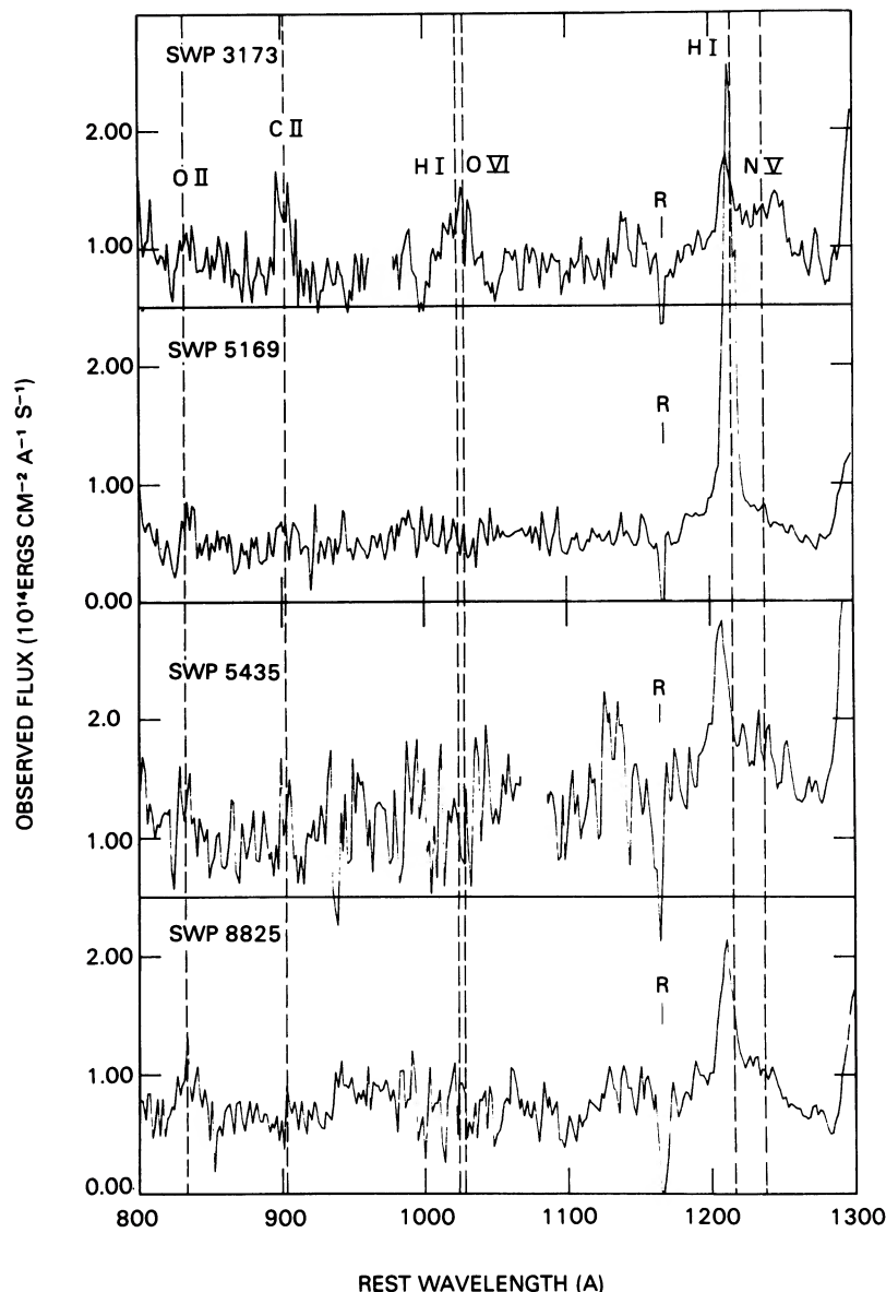
FIG. 1.—Four reextracted IUE spectra of 3C 232 acquired with the Short Wavelength Prime (SWP) camera. The wavelength scale is that of the rest frame of the QSO, assuming a z = 0.533 . The vertical lines denote laboratory wavelengths of ionic transitions indicated in the top panel. The IUE image numbers are given in the upper left in each panel. The spectral features, most notably that of H I–Ly \alpha , may not be perfectly aligned since the quasar may not necessarily be centered on the dispersion axis of the large aperture. Wavelength shifts as large as 4–5 Å might be expected. The peak intensity of H I–Ly \alpha in SWP 5169 is somewhat uncertain since the pixels near the peak flux of this feature are affected by saturation.
