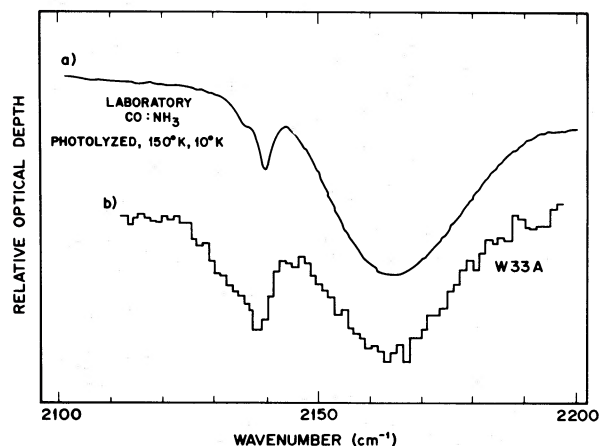
FIG. 5.—The final laboratory spectra of photolyzed \text{CO}:\text{NH}_3 which has been cycled through 150 K (same as Fig. 4e), compared with the spectrum of W33A. The optical depth scale is arbitrary.
