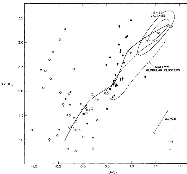
FIG. 10.—Reddening-corrected colors (V-K)_0 and (U-V)_0 are plotted for LMC and SMC (flagged points) clusters. Struck-Marcell and Tinsley's (1978) single burst model is shown as the heavy line; ages in 10^9 years are given along the locus. The regions occupied by M31 and Milky Way globular clusters (Frogel, Persson, and Cohen 1980b) and by E and S0 galaxies (Frogel et al. 1978) are shown. For the latter, the greatest concentration of galaxy points occurs in the inner region; the outer region encloses nearly all our galaxy data. A reddening vector and representative \pm 1 \sigma_m error bar are also given.
