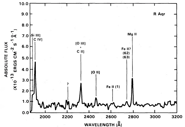
FIG. 2.—Low-dispersion spectrum of R Aqr between 2000 and 3200 \text{\AA} obtained with the large aperture on IUE . Exposure time was 20 minutes. The feature identified with a question mark is probably an artifact in the detector. The continuum level is seen to rise slightly toward long wavelengths.
