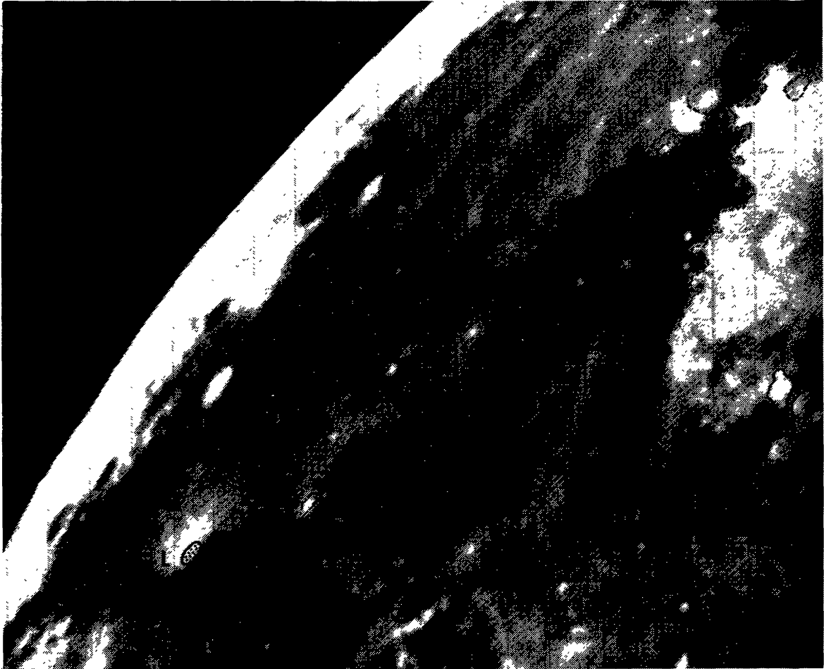
Fig. 5. Full Moon photograph of Sinus Roris and northern Oceanus Procellarum, showing covering of ray systems by bluer material, and correspondence between the sinuous rille Rima Sharp I and the bluest region. A, region of very 'blue' material; B, region of less 'blue' material; C, abrupt cut-off of rays from Pythagoras; D, abrupt resumption of rays; L, Lichtenberg and half-covered ray system; R_S Rima Sharp I and its source S_S ; R_M , anonymous rille, named here the Mairan rille, and its source S_M ; M, 'red' mountains, Gruithuisen gamma and delta.
