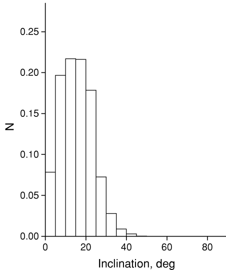
Figure 4. The steady-state i distribution for Centaurs captured from the NNHE region over 100 Myr.
