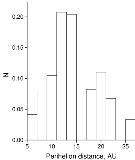
Figure 9. The debiased q distribution for observed Centaurs with a < 60 au assuming q' = 4 for H < 8 and q' = 1 for H > 8 .
