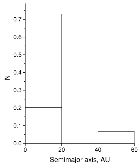
Figure 8. The debiased a distribution for observed Centaurs with a < 60 au assuming q' = 4 for H < 8 and q' = 1 for H > 8 .
