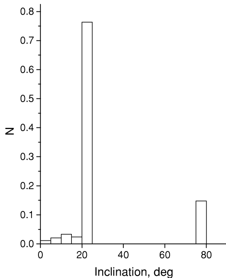
Figure 7. The debiased i distribution for observed Centaurs.
