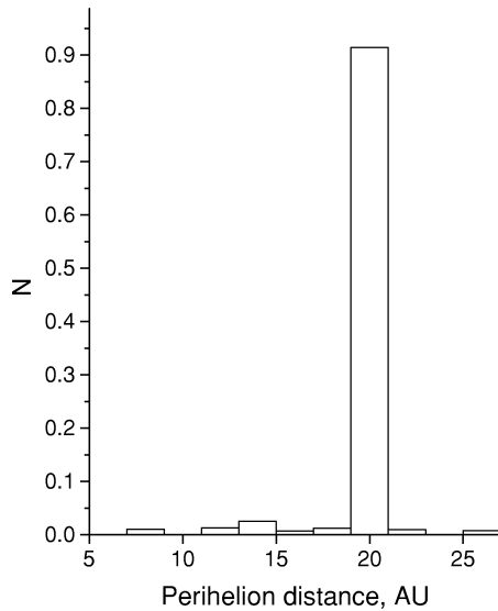
Figure 6. The debiased q distribution for observed Centaurs.
