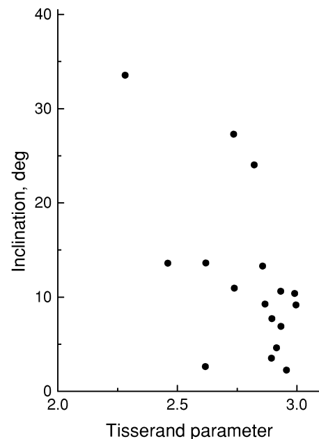
Figure 10. The distribution of Tisserand parameters and inclinations for simulated objects from the region 5 < q < 28 au, a > 60 au when their perihelia first drop below 2.5 au.
