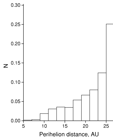
Figure 3. The steady-state q distribution for Centaurs captured from the NNHE region over 100 Myr.
