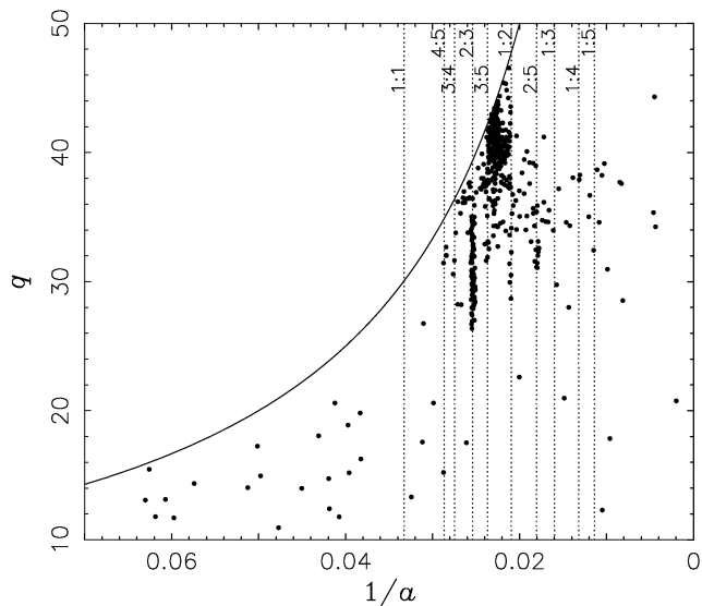
Figure 1. Observed distribution of multiple-opposition TNOs and Centaurs (2005 February). The solid curve shows the locus of objects of zero eccentricity. Dotted lines show the principal mean-motion resonances with Neptune. Note the absence of non-resonant objects with q close to the orbit of Neptune and a \lesssim 50 au.
