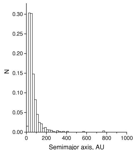
Figure 2. The predicted a distribution for Centaurs captured from the NNHE region over 100 Myr. N denotes the fraction of objects lying in each bin of the histogram.
