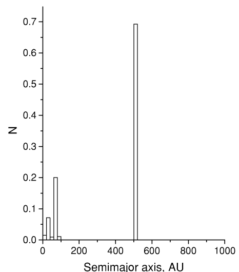
Figure 5. The debiased a distribution for observed Centaurs.
